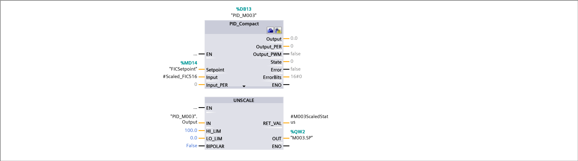
Network 9: Valves
