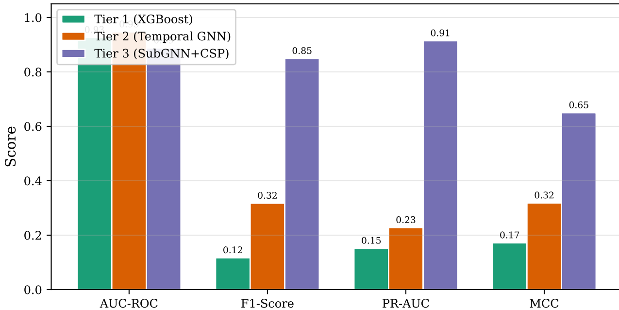
(a) Classification Metrics by Tier
