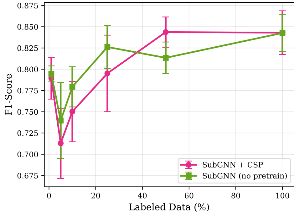
(b) F1-Score vs. Label Fraction
