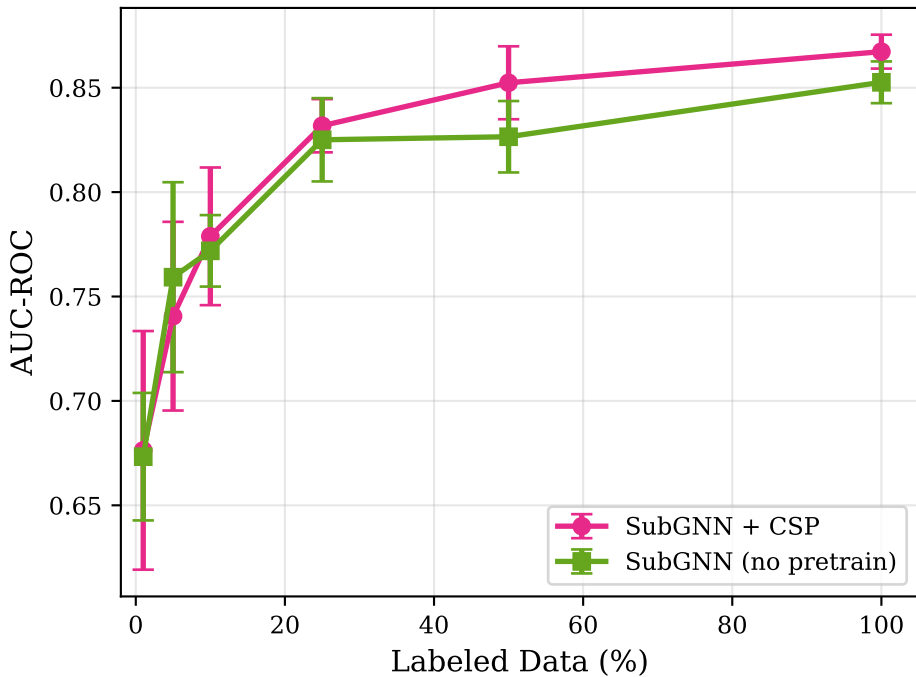
(a) AUC-ROC vs. Label Fraction
