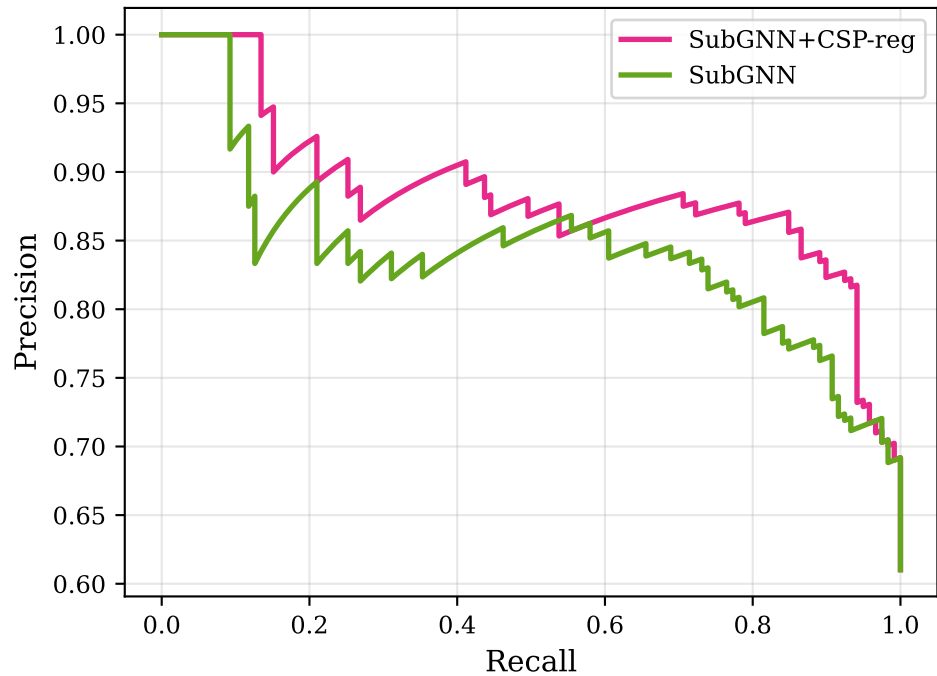
(b) Precision-Recall Curve
