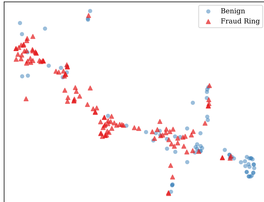
SubGNN
