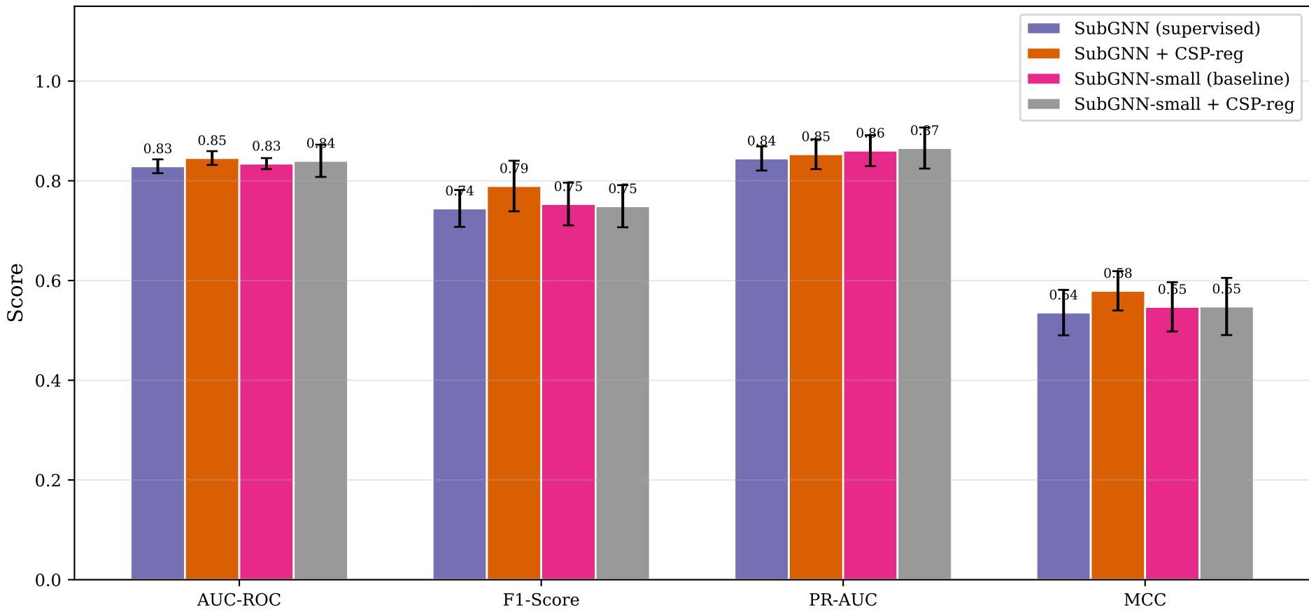
Ablation Study: Component Contributions (mean \pm std, n=5 runs)
