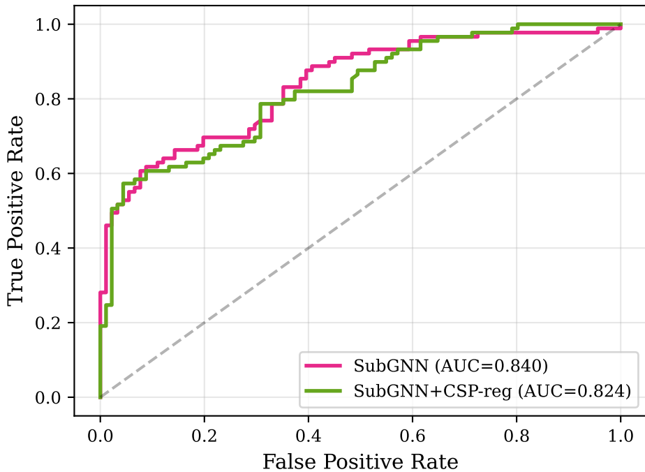
(a) ROC Curve
