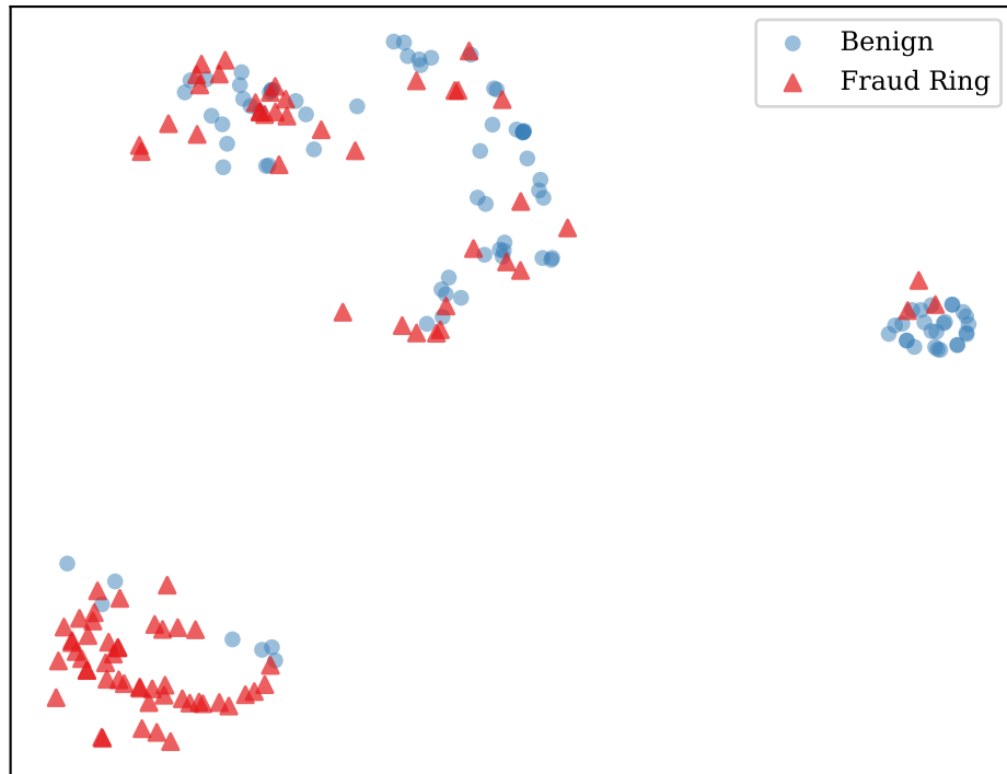
SubGNN
