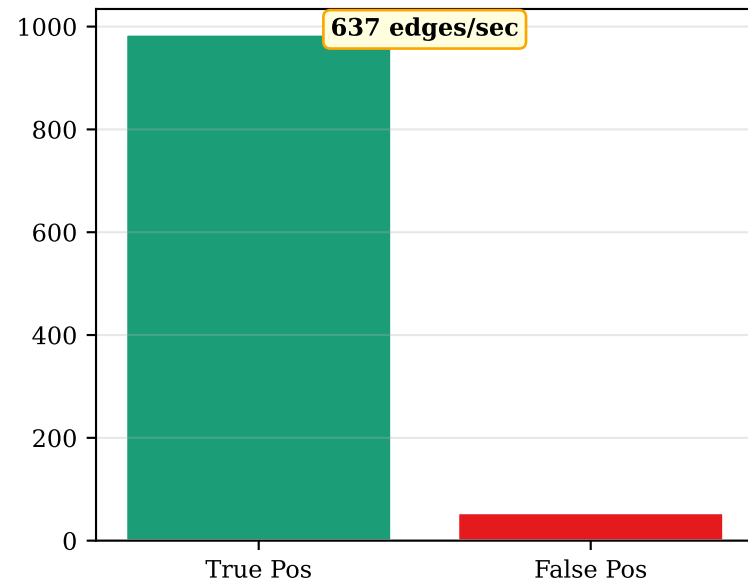
(c) Precision: 94.8%
