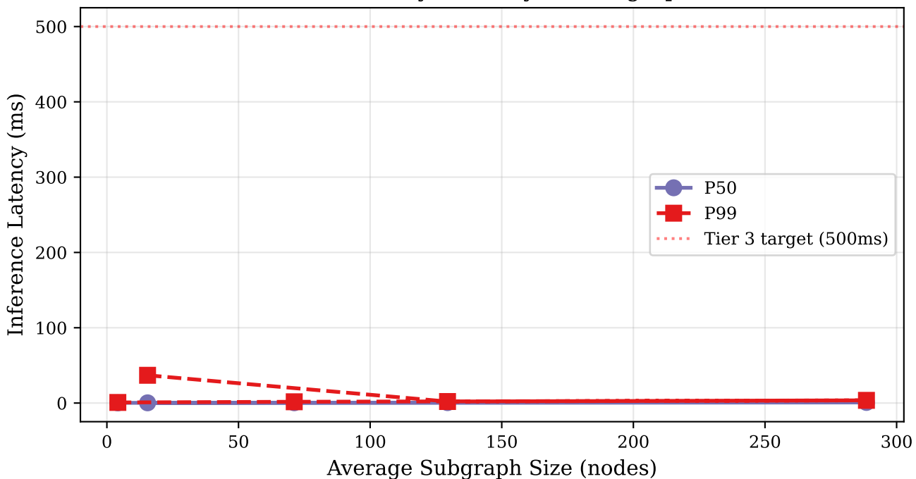
Tier 3 Scalability: Latency vs. Subgraph Size
