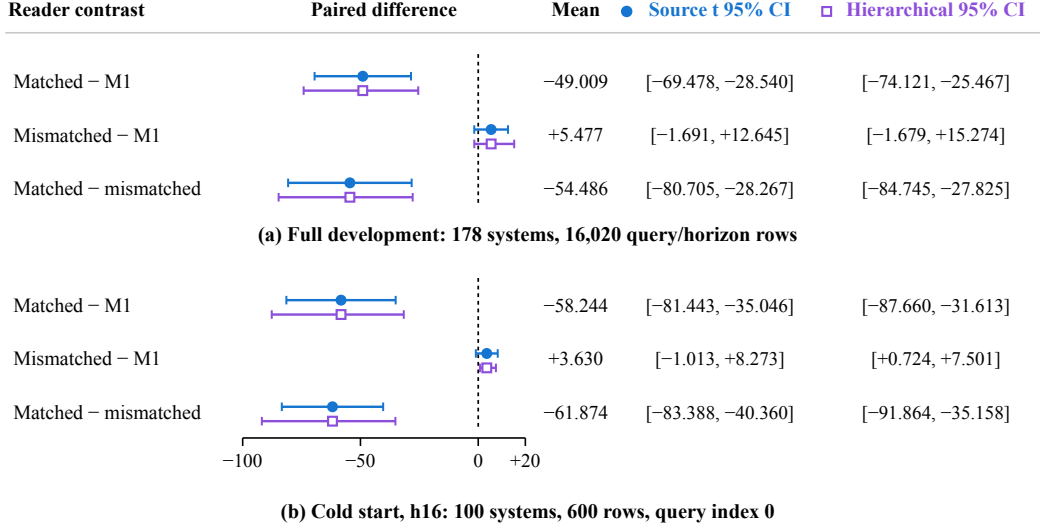
Figure 23: Paired error differences for the matched-architecture control. (a) Full development mixture; (b) cold-start h16. Negative values favor the first reader ( 10^{-3} MSE). Source-paired 95% t intervals use three source means; hierarchical 95% intervals resample sources, readers and systems. Both condition on development-selected fits; matched and mismatched M_2 readers are fitted separately.
