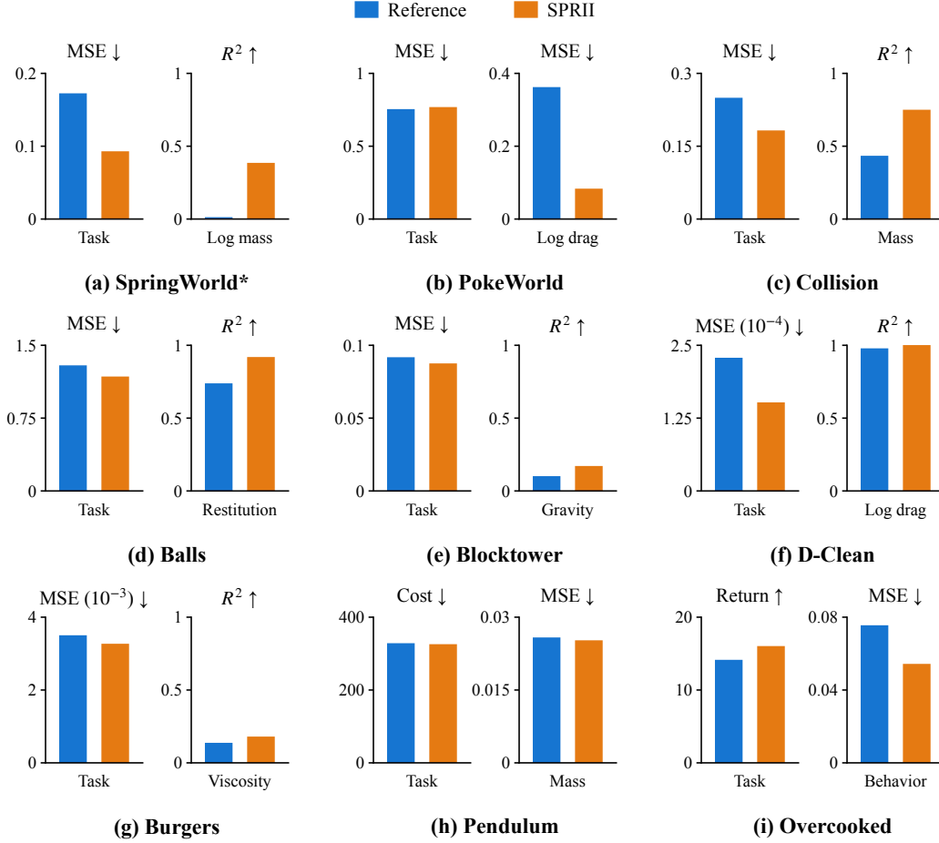
Figure 7: Original-metric task and property comparisons. Left: task; right: property. Blue: reference; orange: SPRII; arrows indicate preferred directions. Comparisons are (a) Native JEPA → Align + Cross; (b) random → correct pairing; (c) Native CPC → Cross; (d) Native RSSM → Cross; (e) Native JEPA → Cross; (f) CaDM → SPRII; (g) Plain CoDA → Cross; (h) CaDM → SPRII; (i) H+VC → Align. Task endpoints are (a) cold-start MSE, (b) h16 state MSE, (c–e) trajectory MSE, (f) h32 MSE, (g) ID MSE, (h) ID control cost and (i) familiar-partner return. Property metrics and targets are labeled in each panel; Collision and Blocktower use independent support S , and Balls uses reader memory M .
