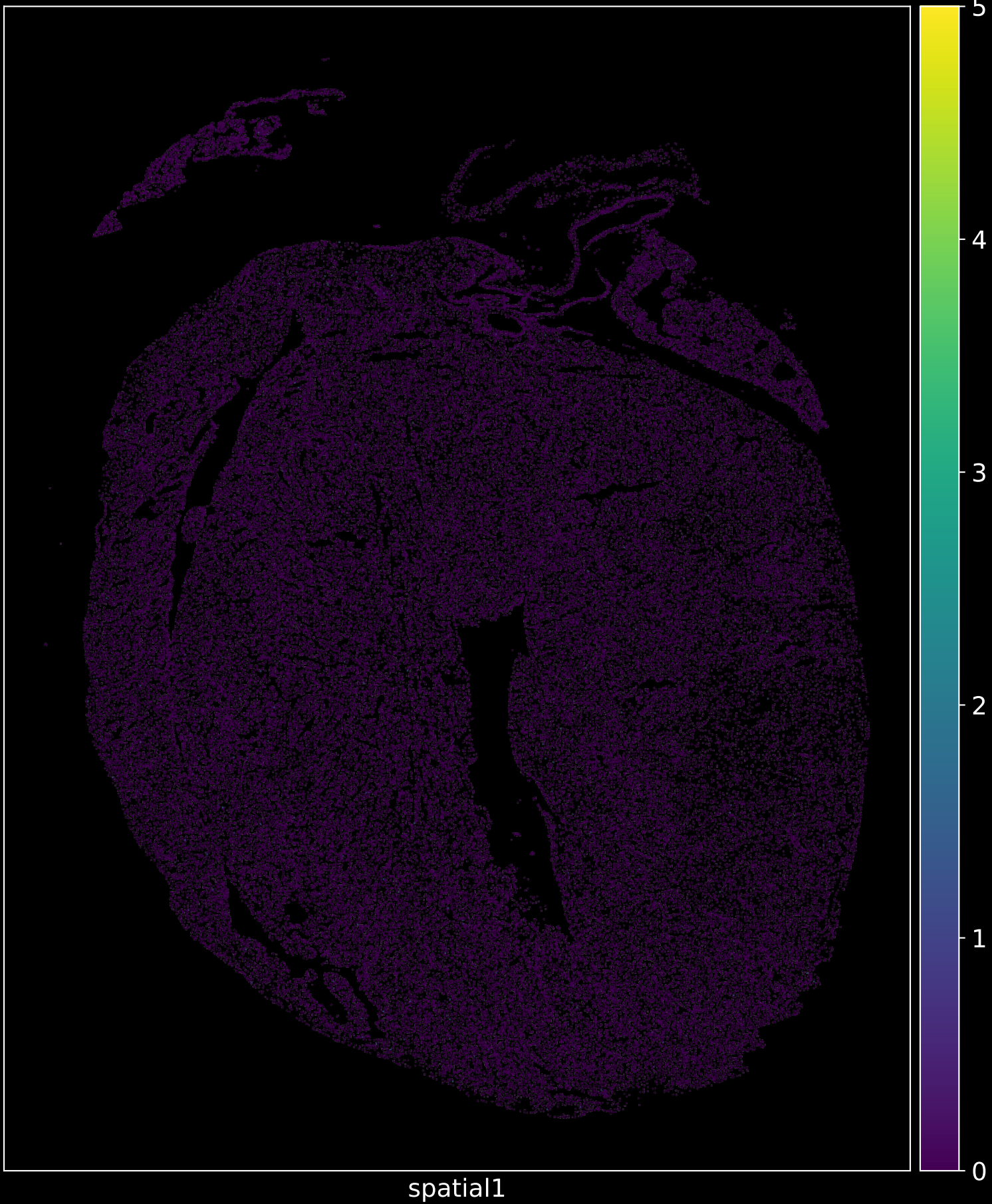
Slamf7 in WT1
