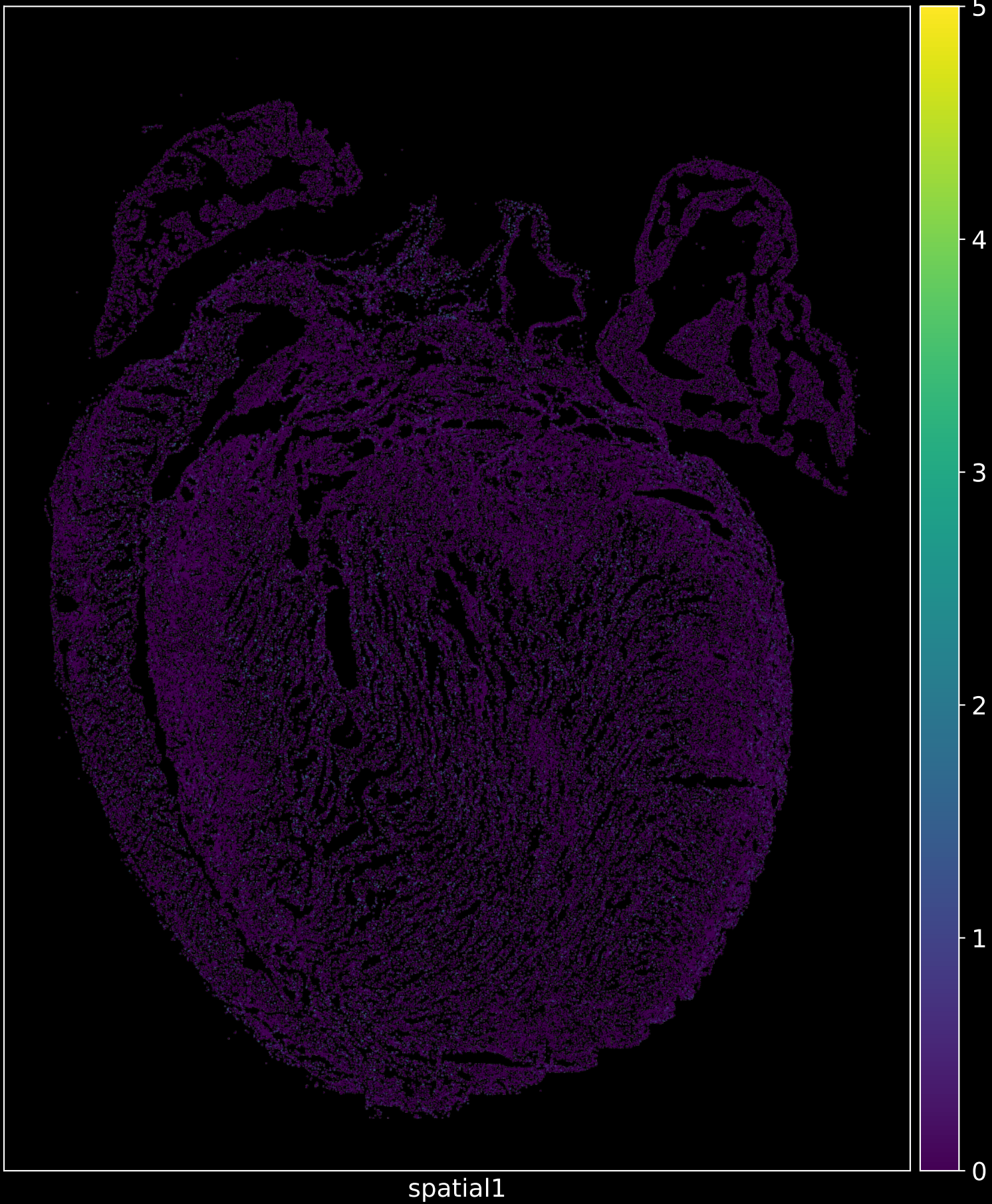
Smoc2 in cKO
