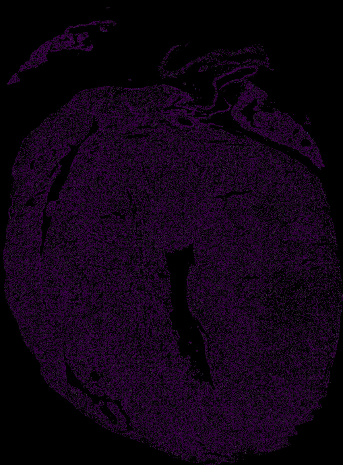
Bnc1 in WT1
