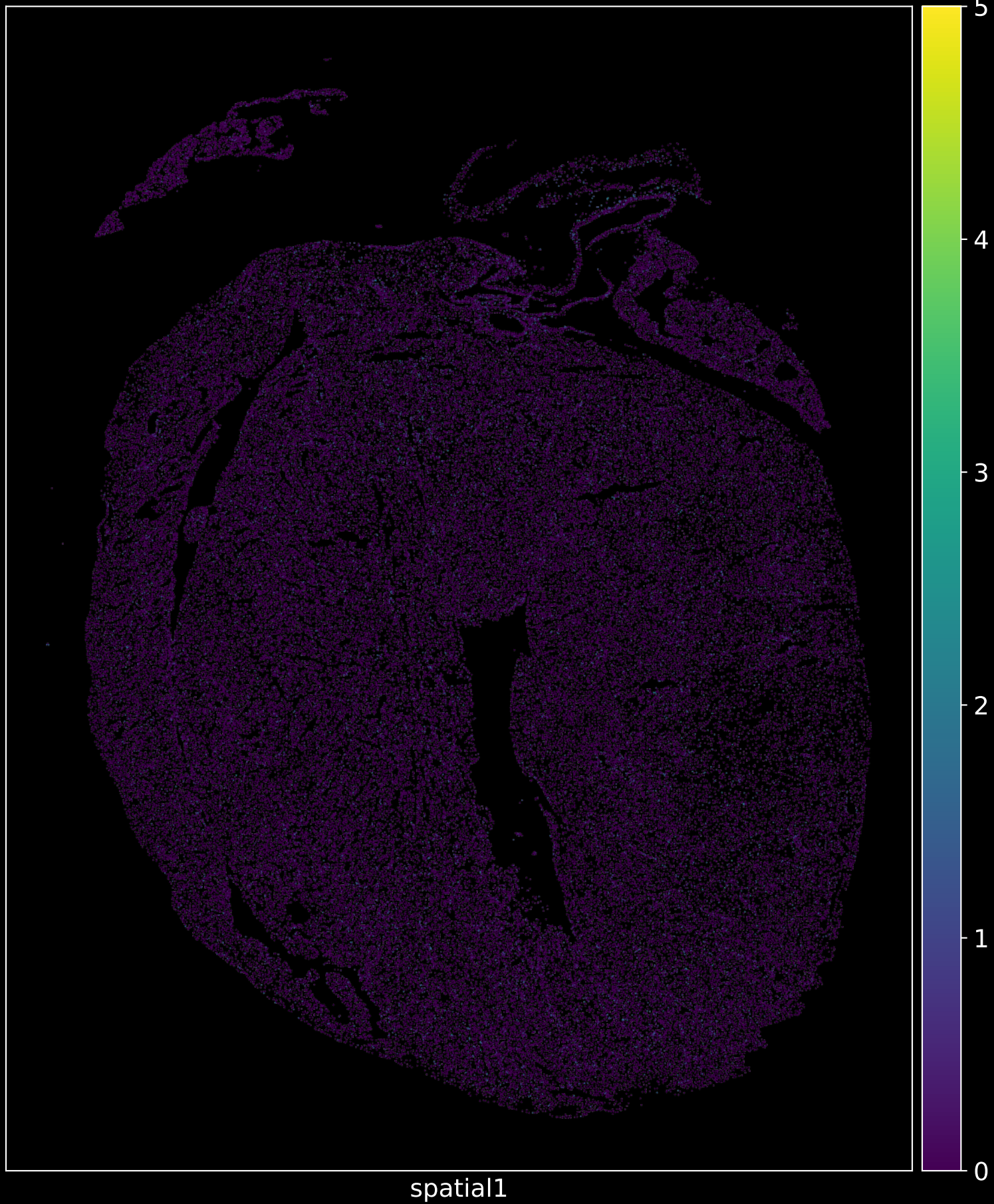
Fbn1 in WT1
