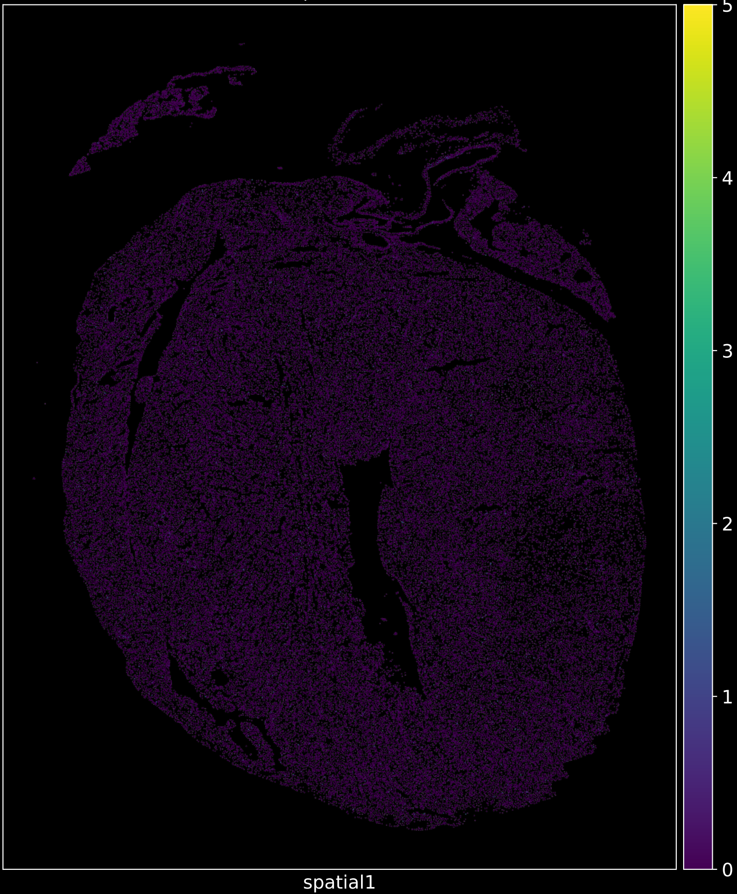
Serpini1 in ctrl
