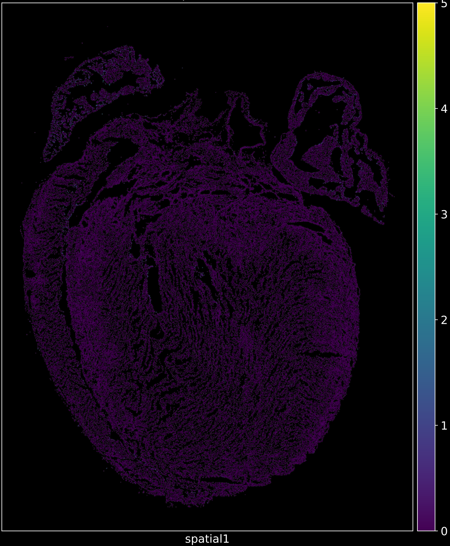
Npr3 in KO1
