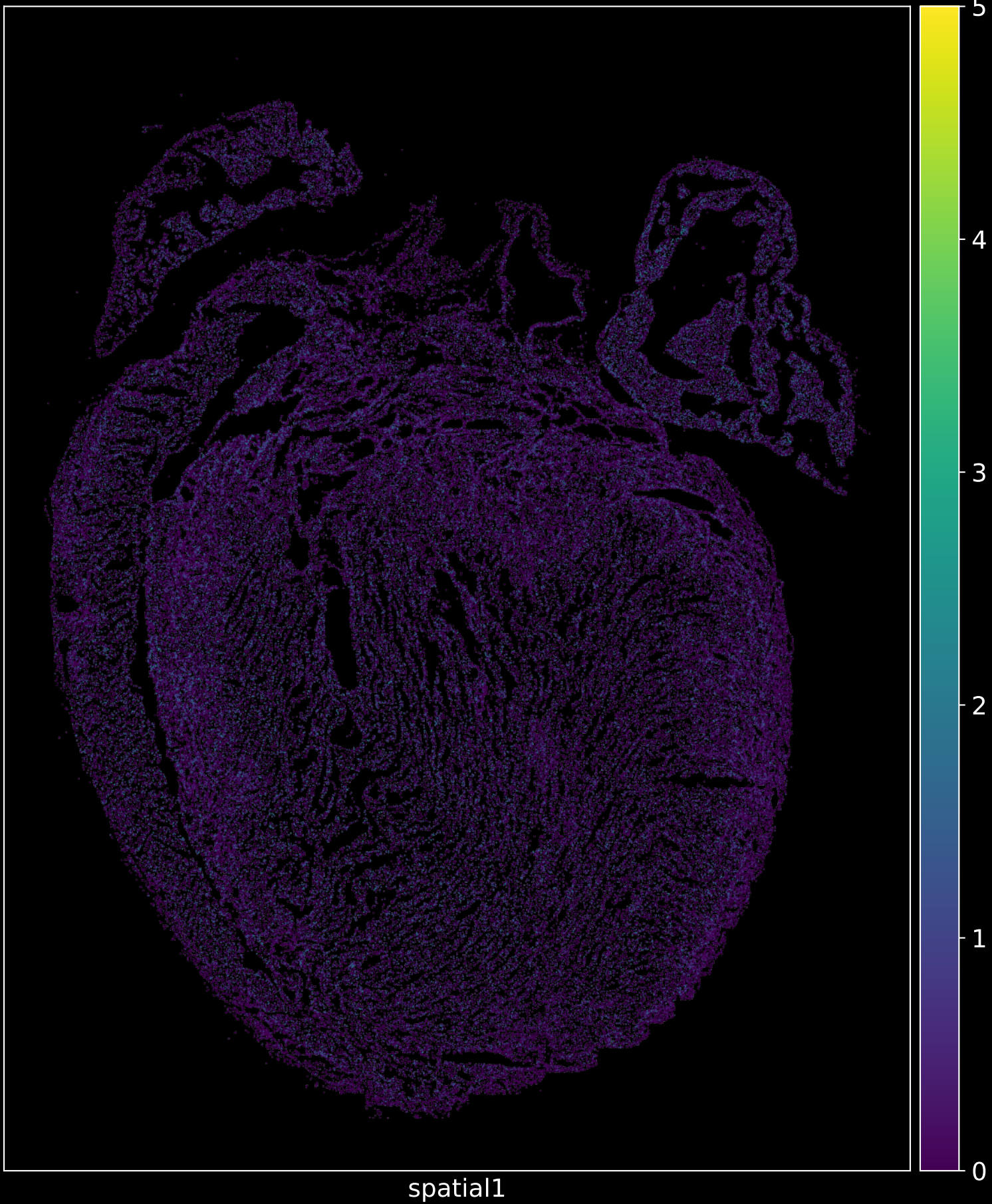
Camk2d in KO1
