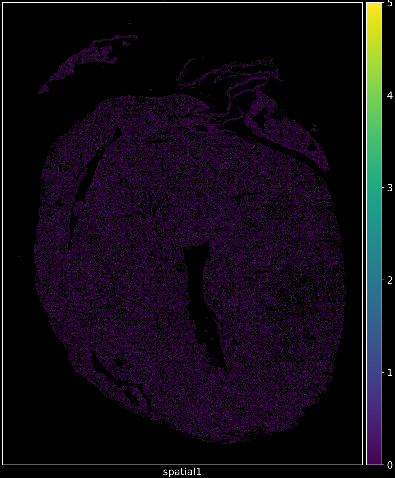
Nrp2 in WT1
