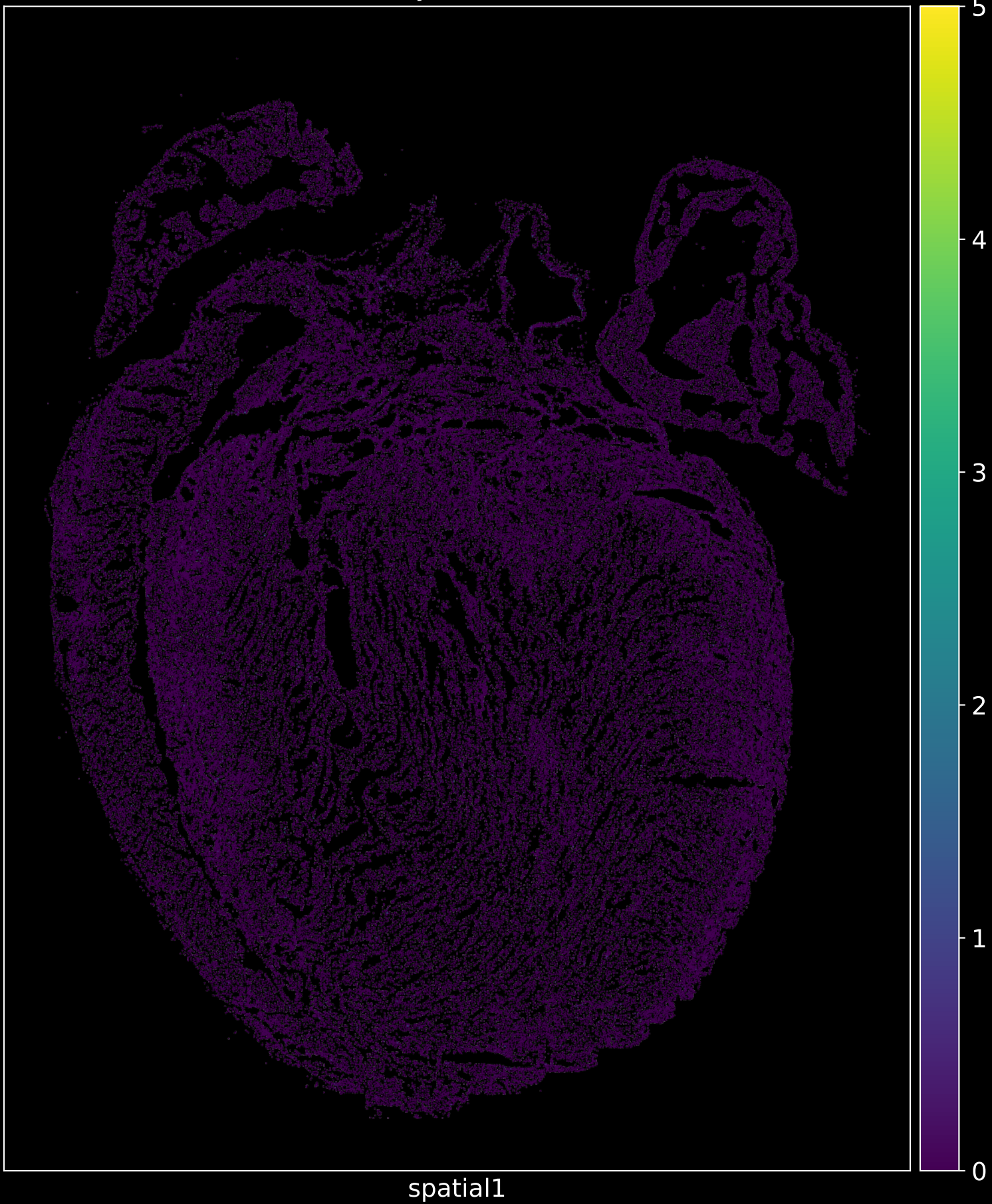
Hey2 in cKO
