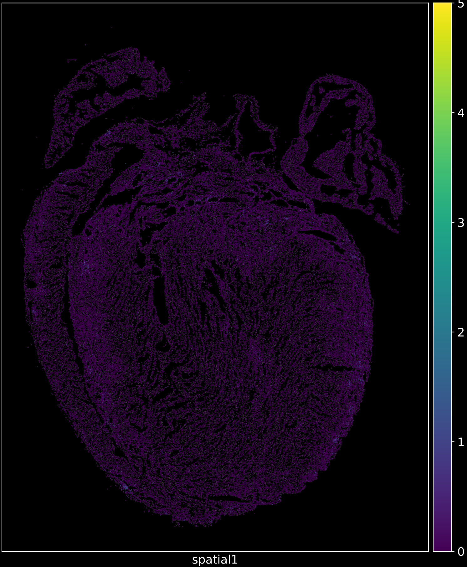
Irf8 in cKO
