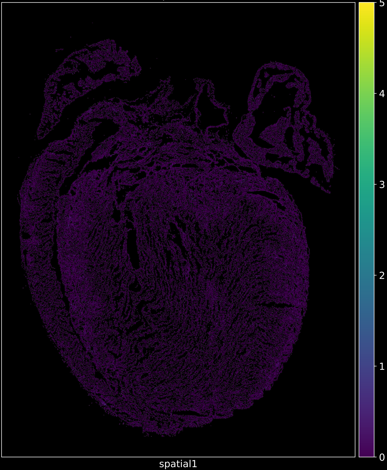
Nlrp3 in cKO
