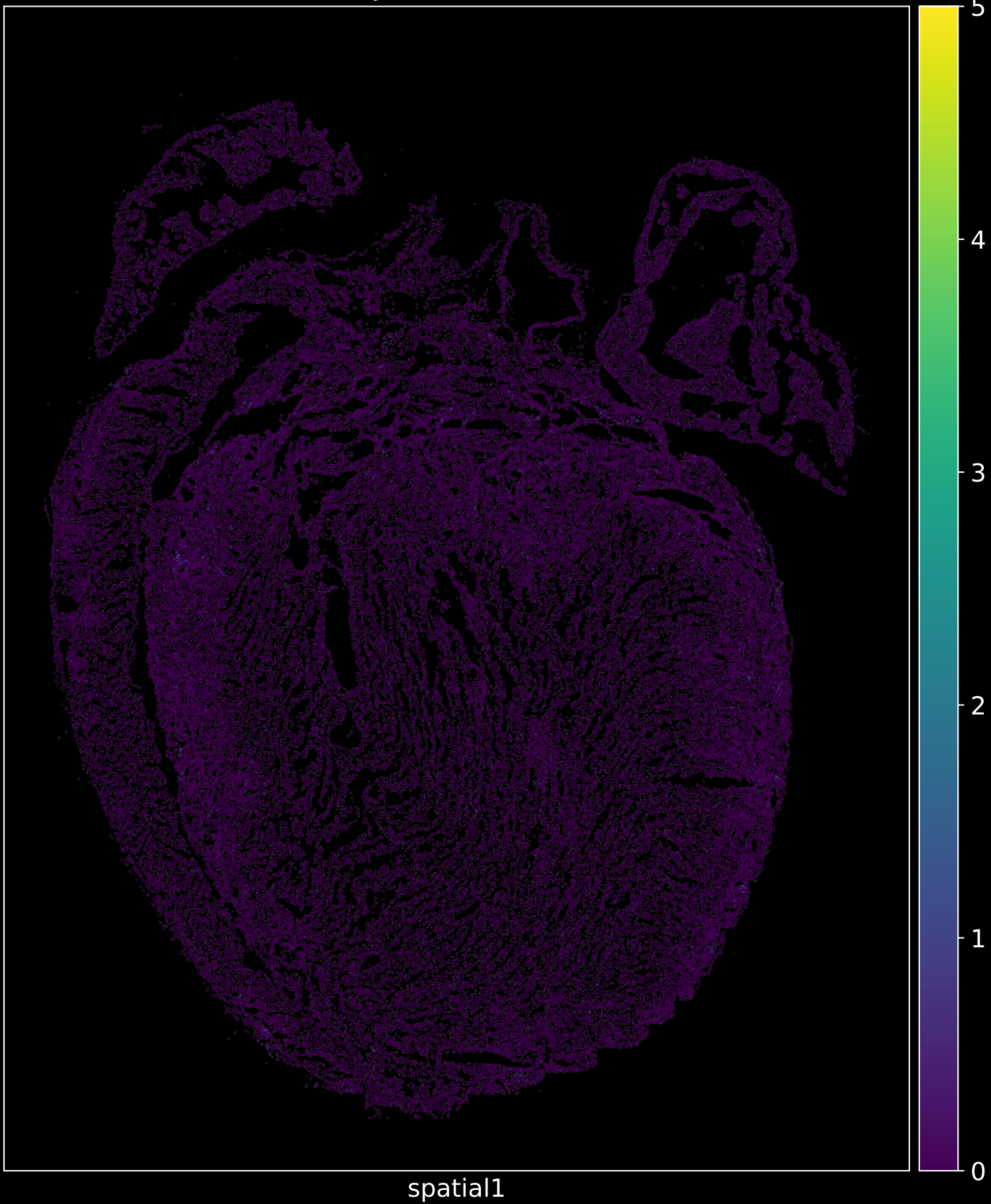
Jchain in KO1
