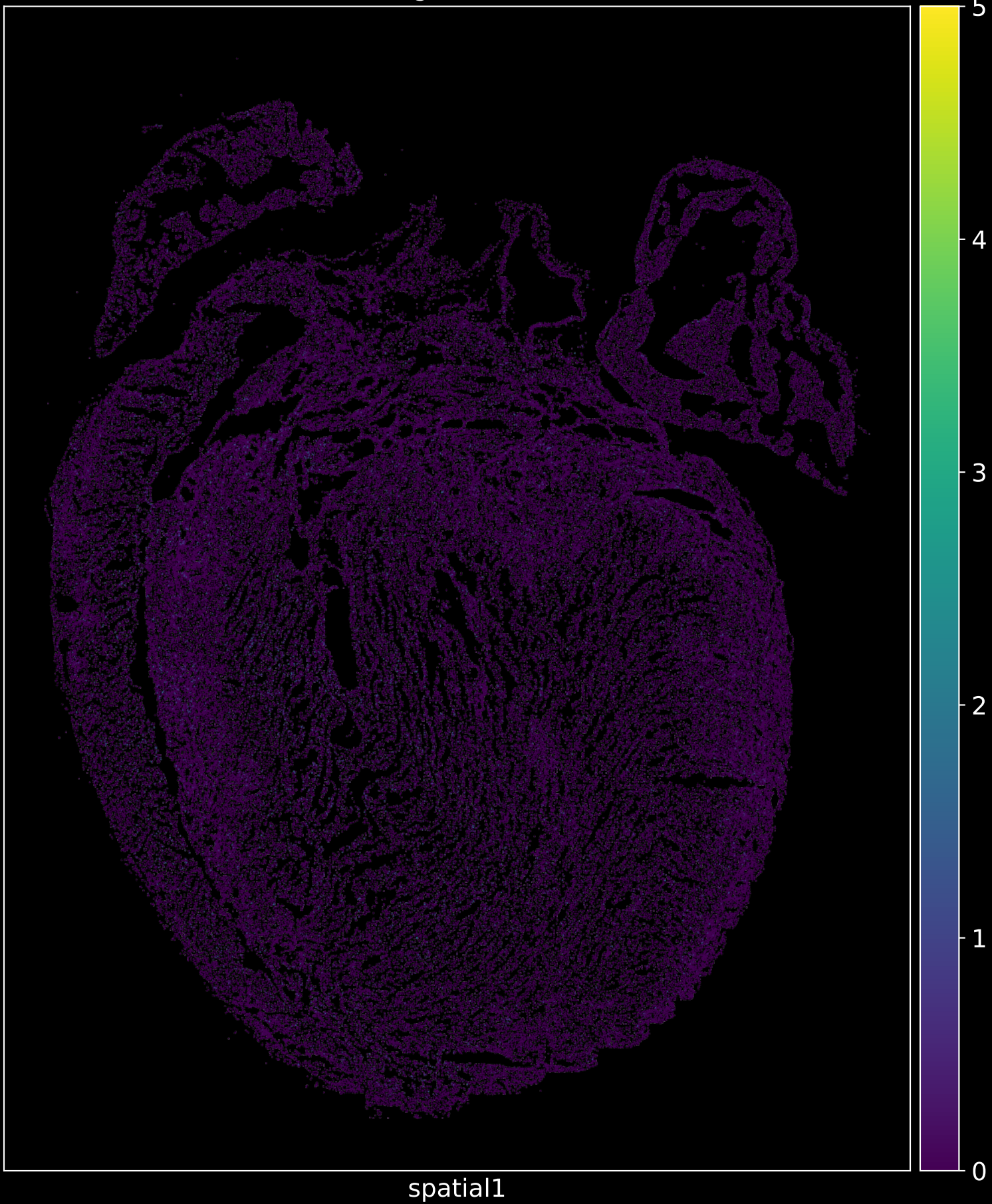
Dsg2 in KO1
