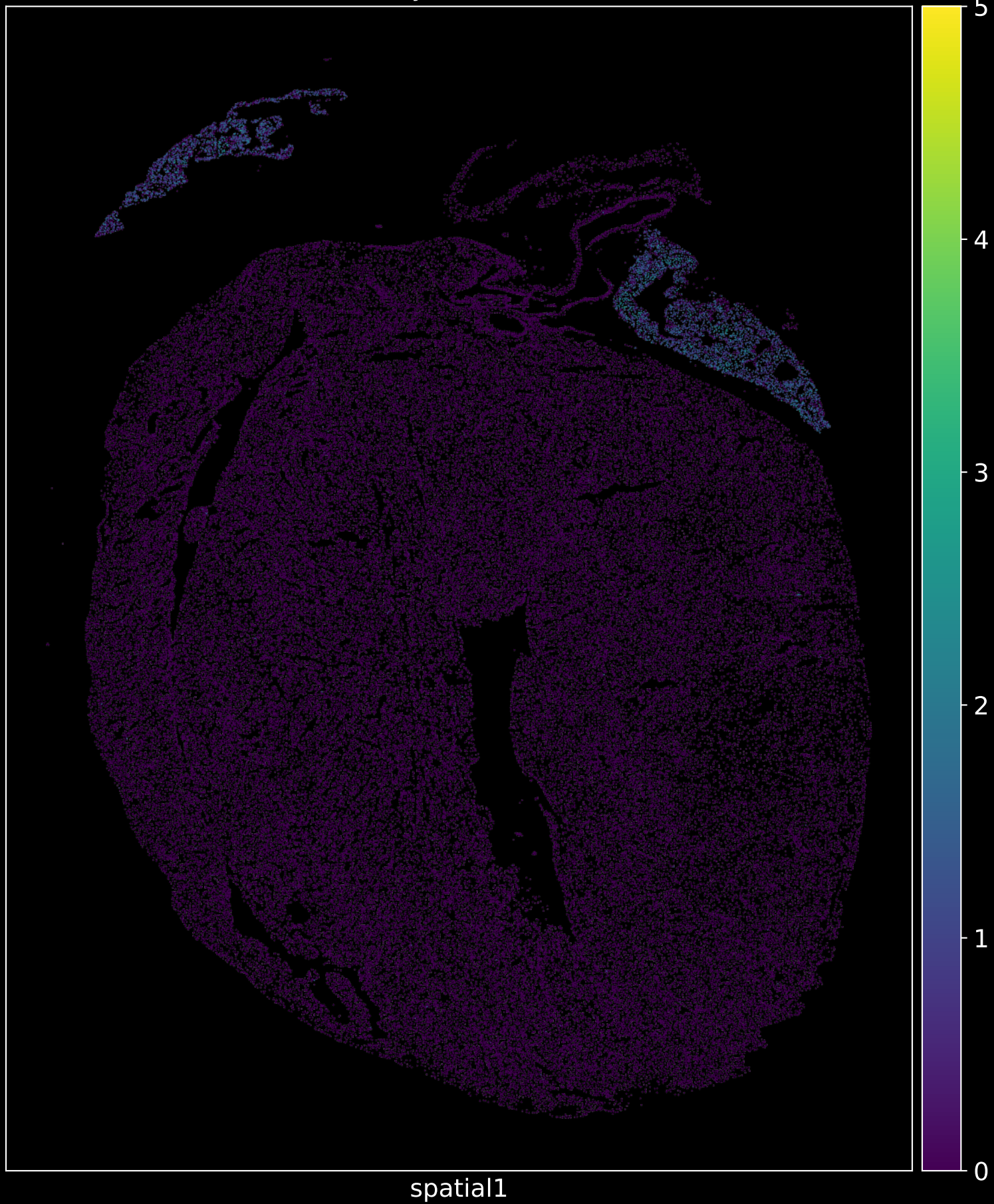
Myl4 in ctrl
