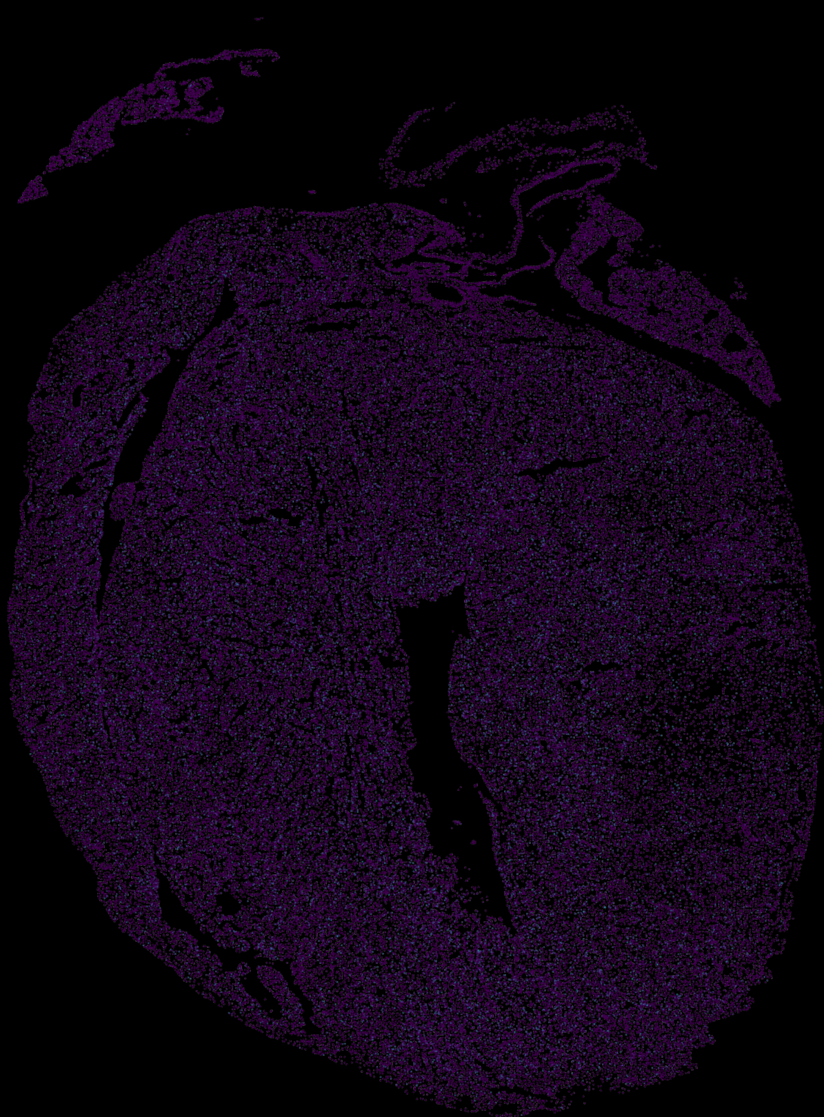
Scn5a in WT1
