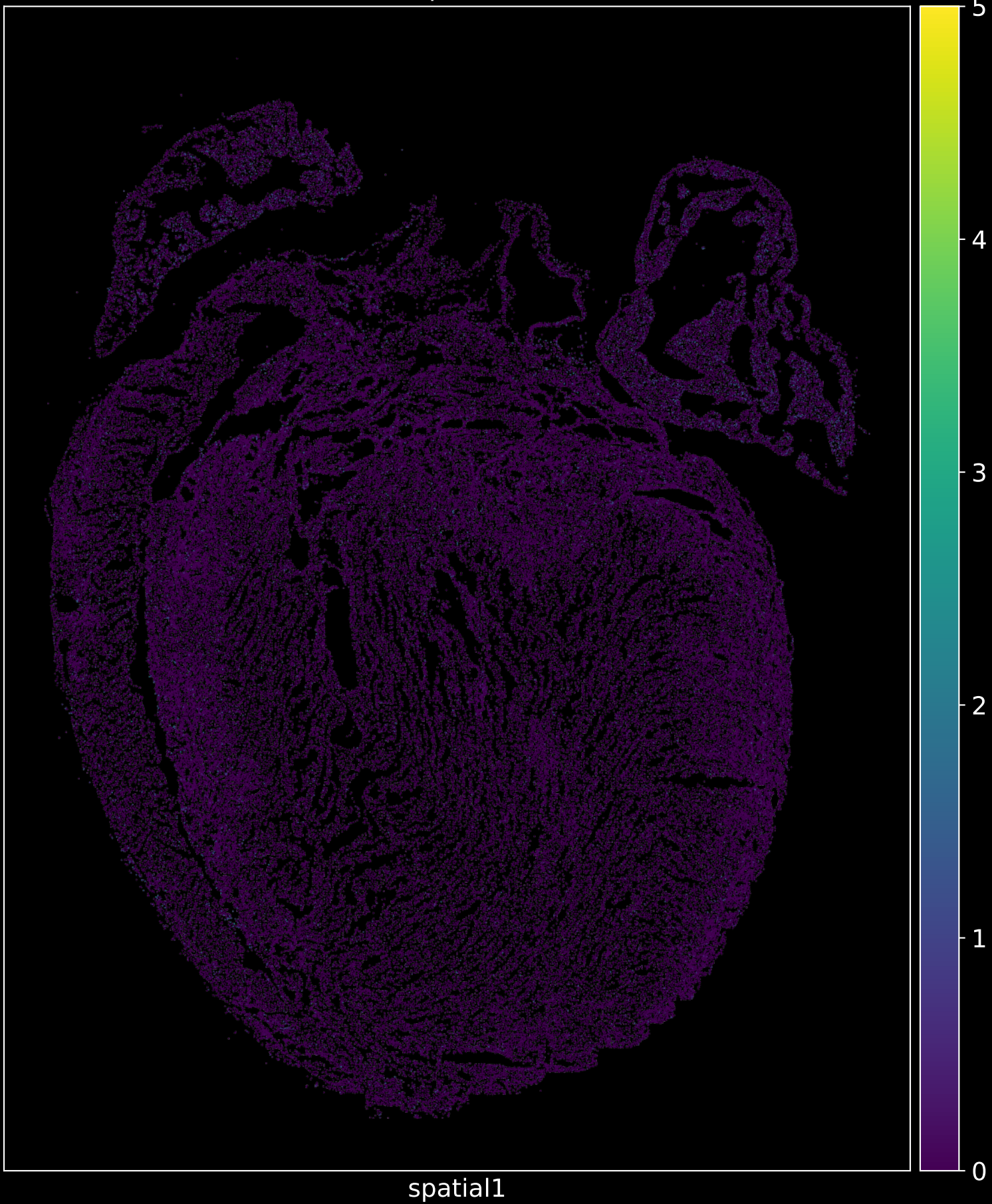
Efemp1 in KO1
