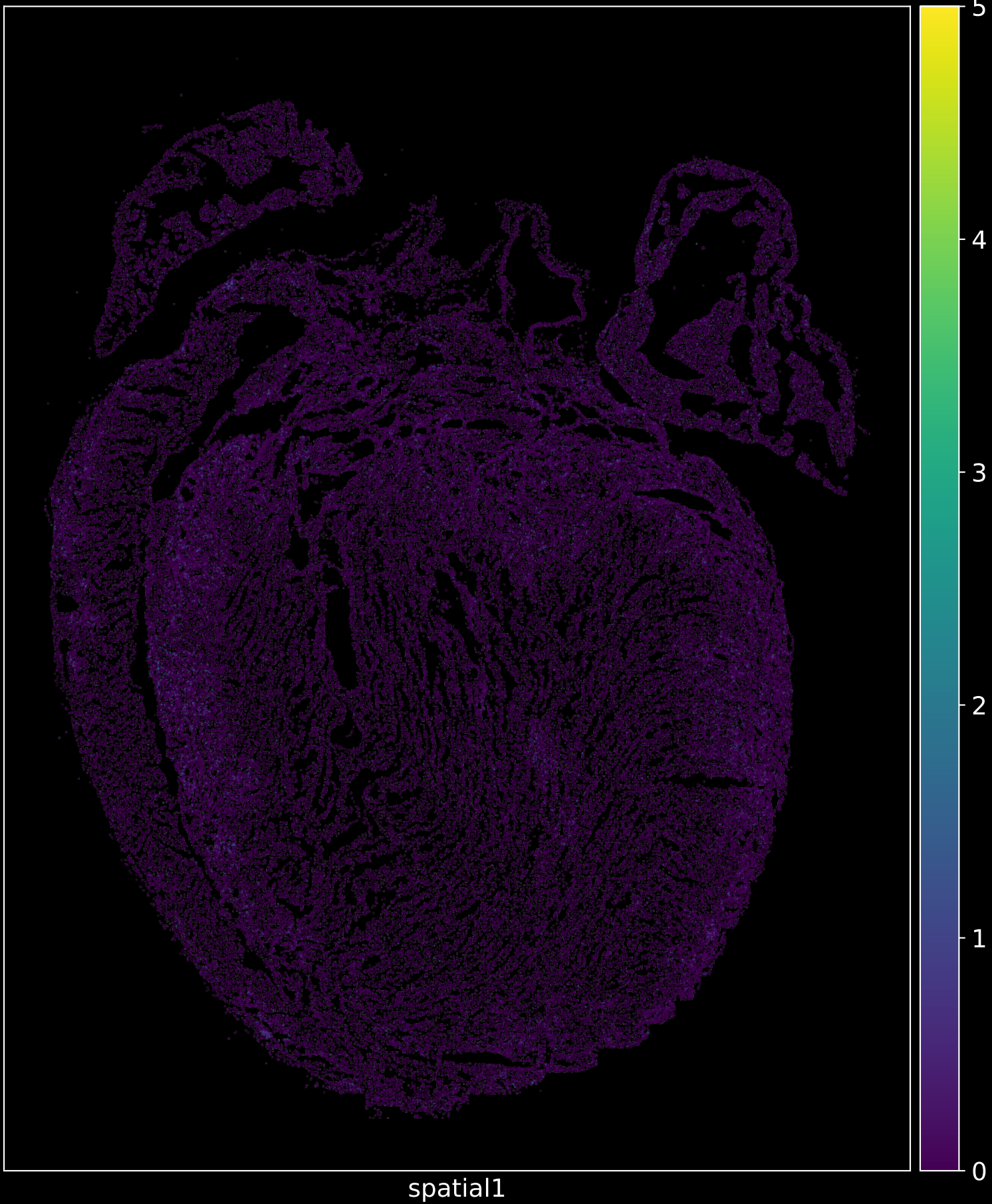
Cd83 in cKO
