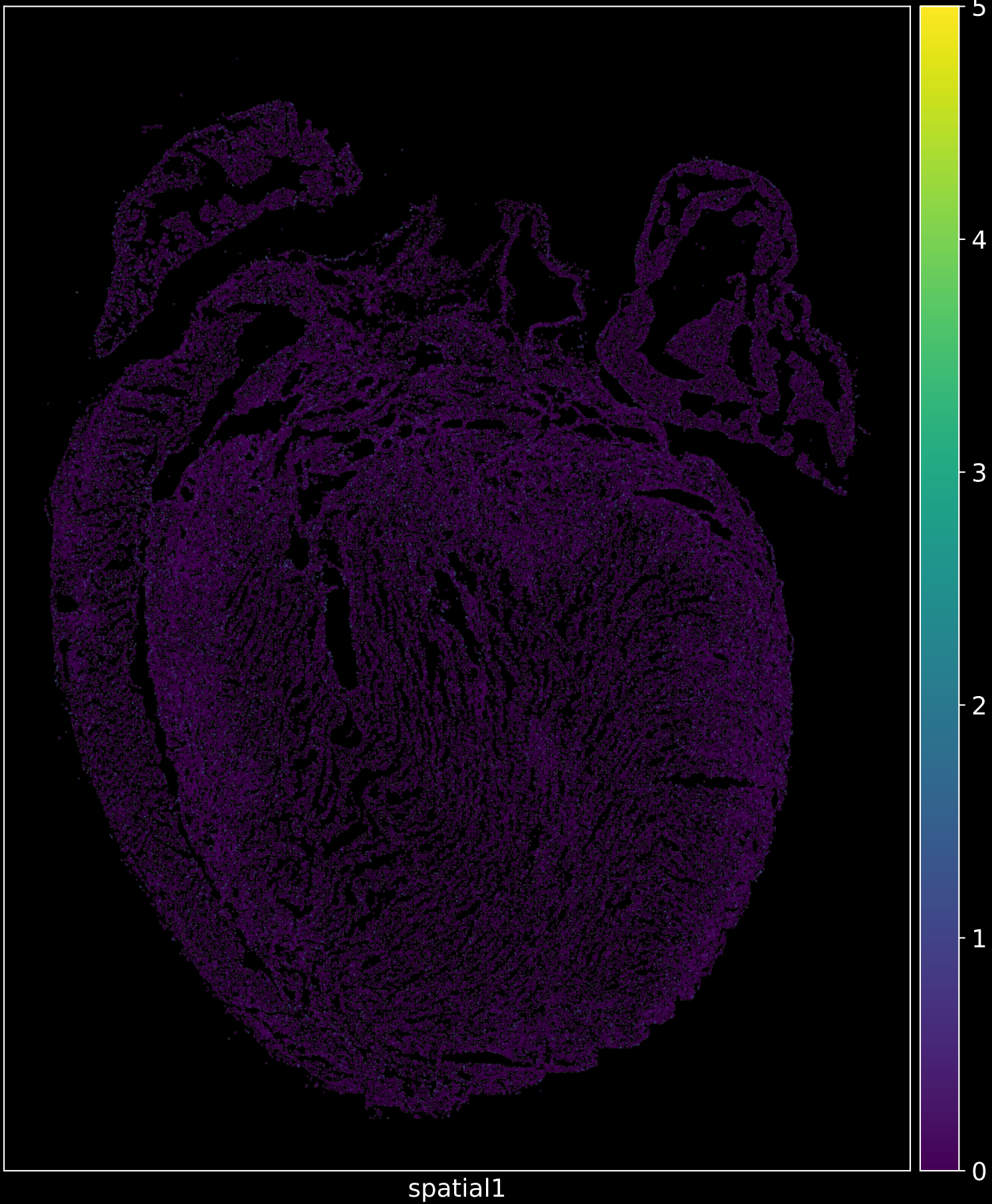
Cdh11 in cKO
