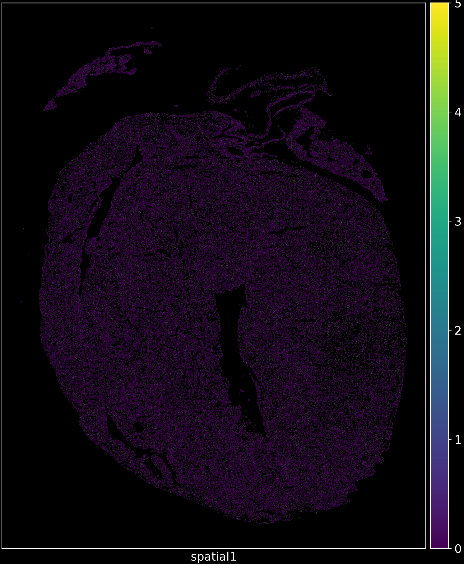
Slc2a13 in ctrl
