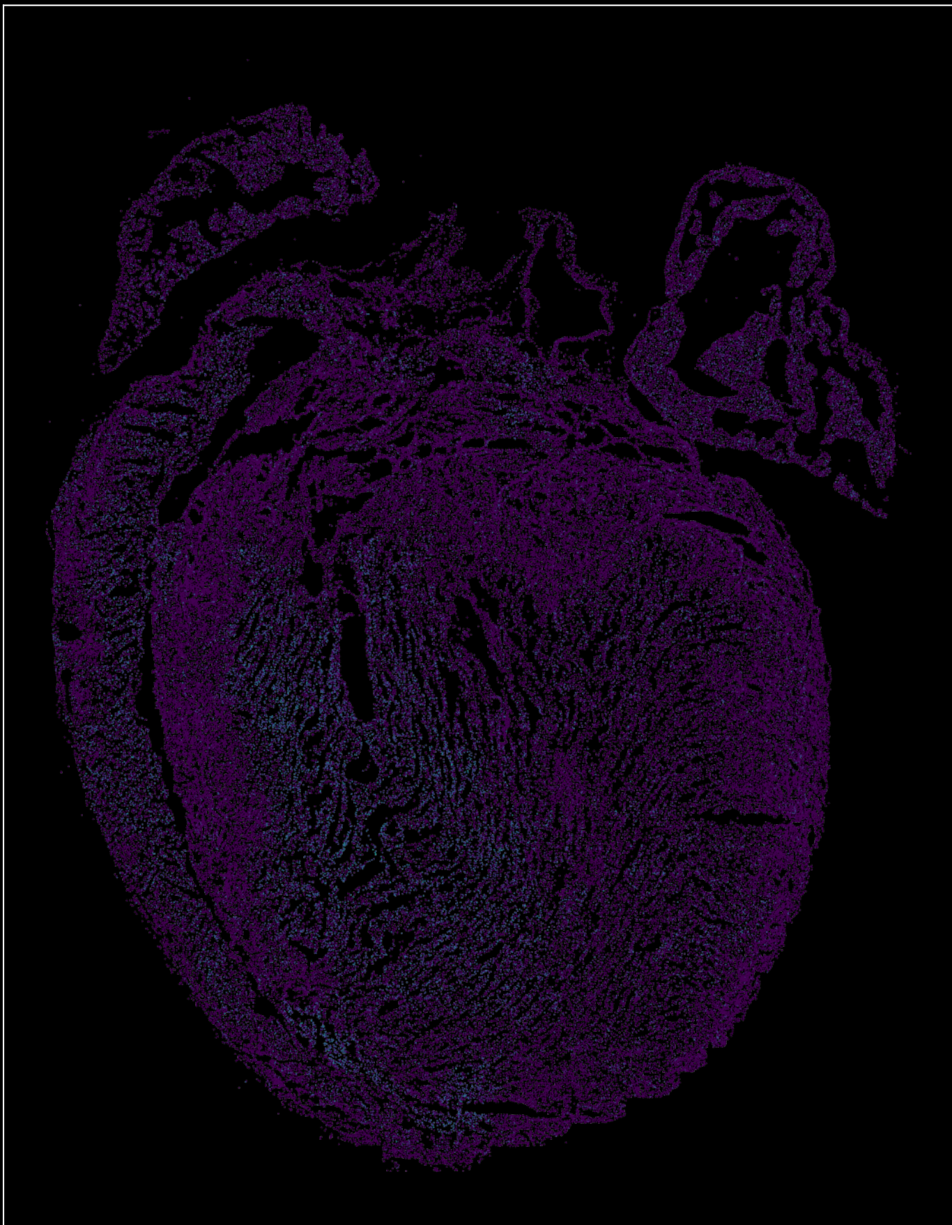
Pdk4 in cKO
