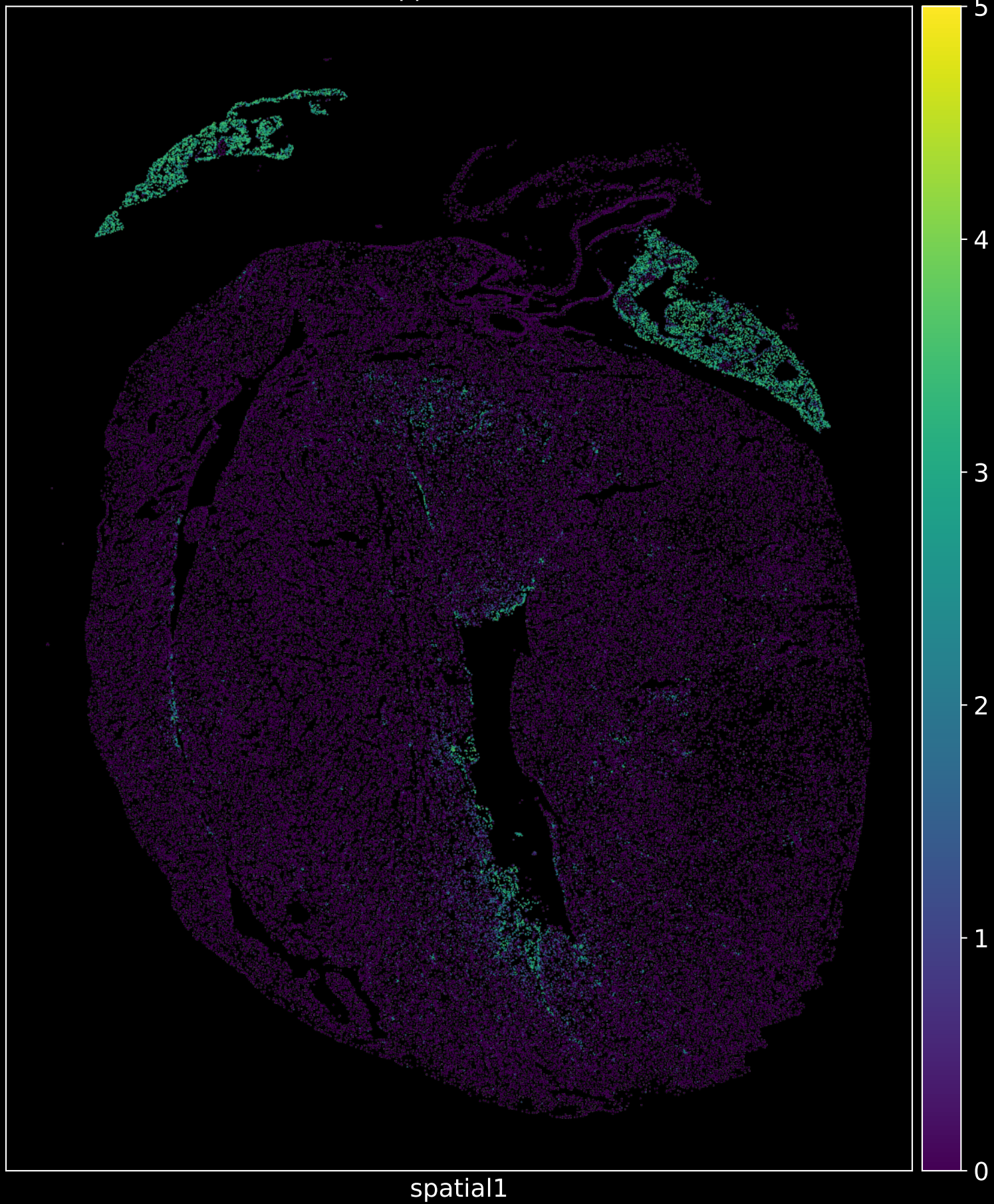
Nppa in WT1
