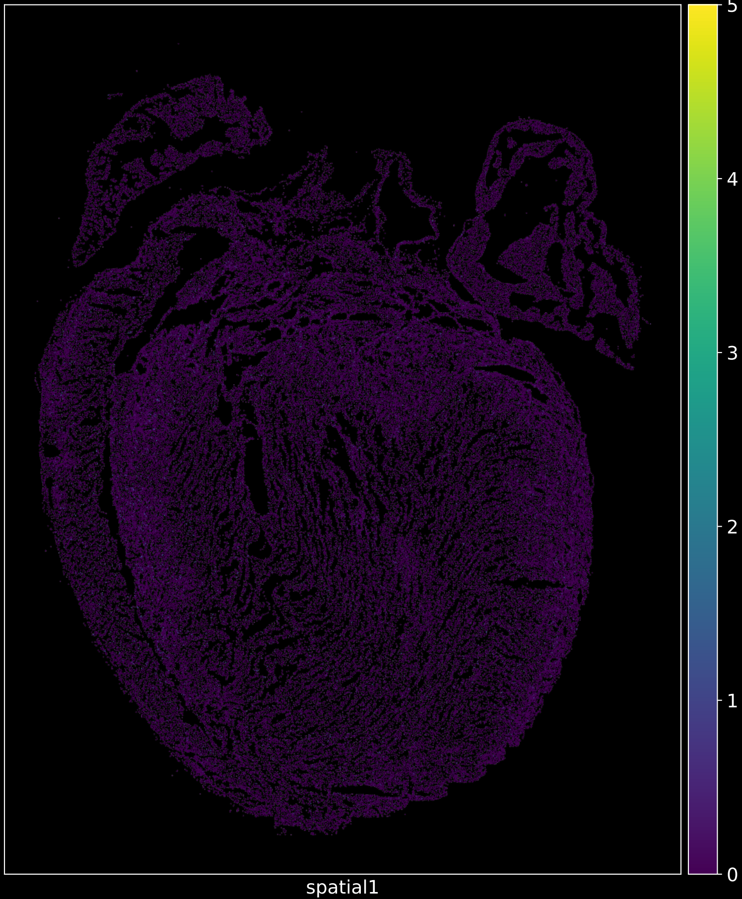
Gsta3 in cKO
