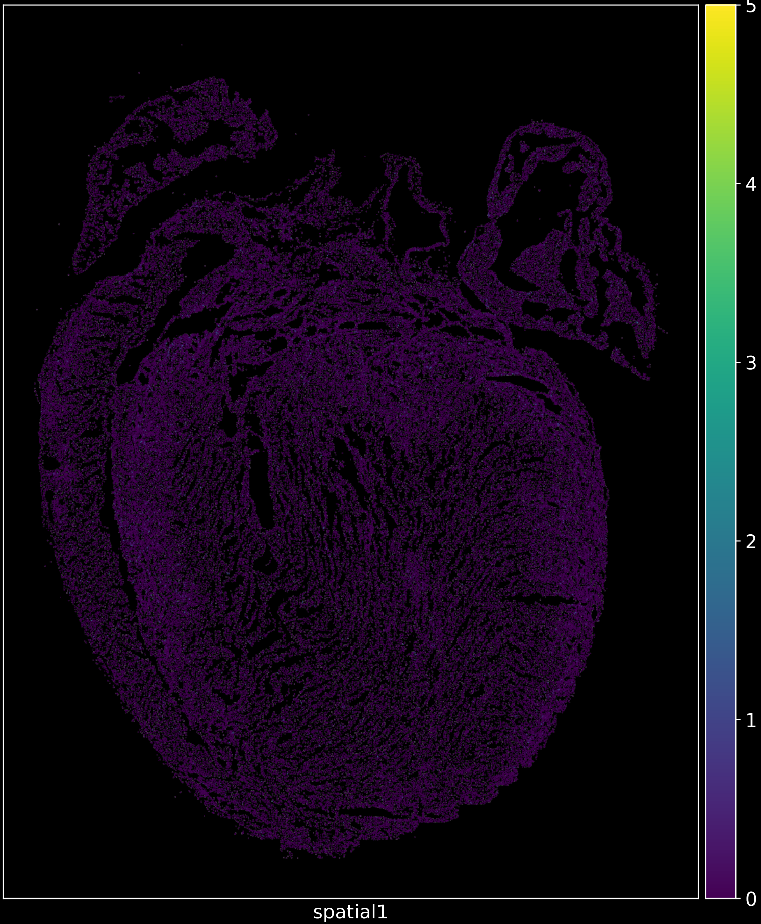
Nrxn1 in KO1
