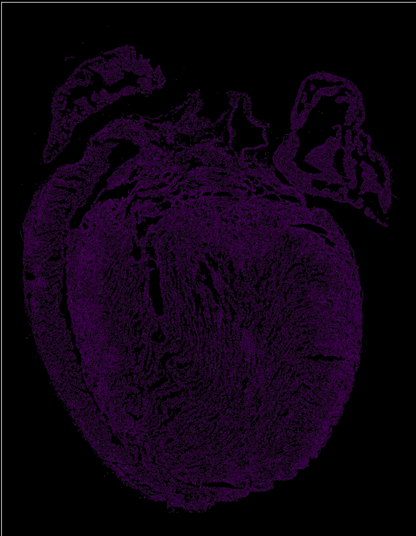
Tgfb2 in cKO
