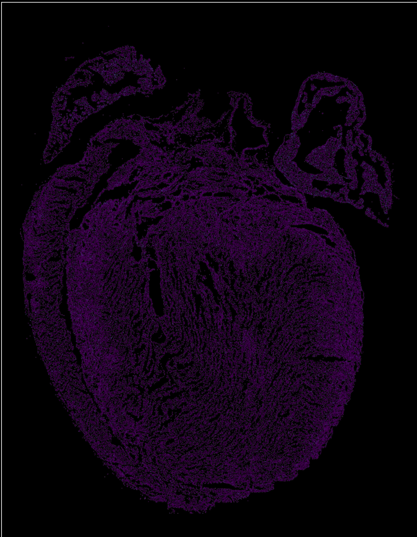
Slc2a13 in cKO
