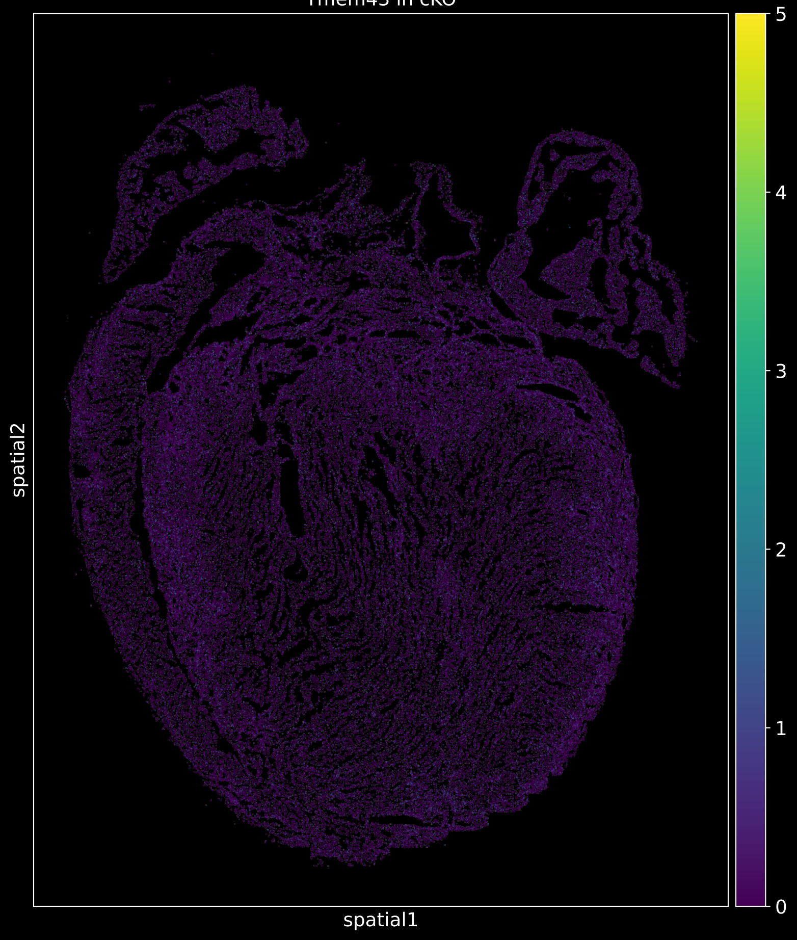
Tmem43 in cKO
