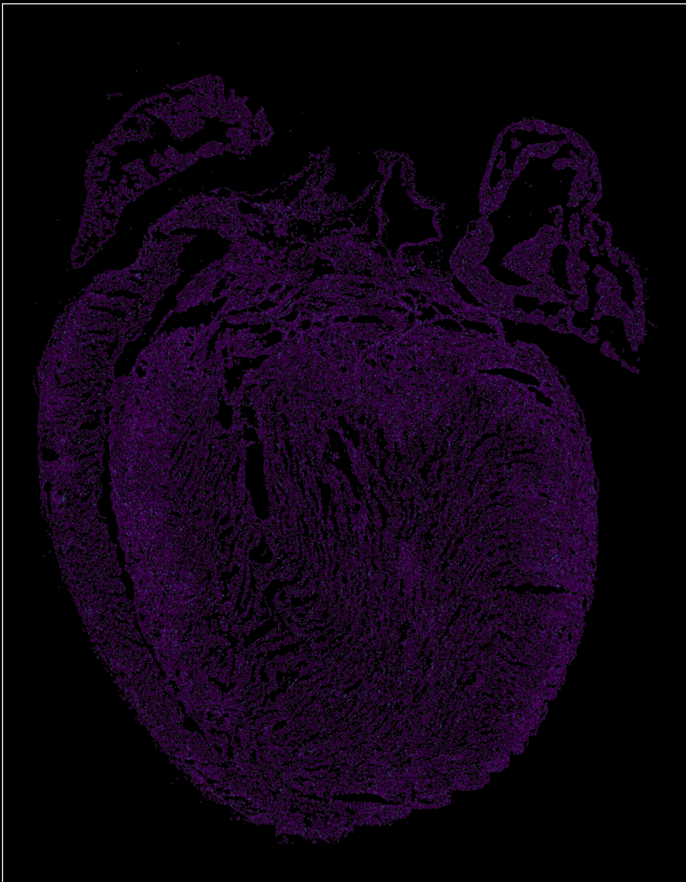
Jag1 in KO1
