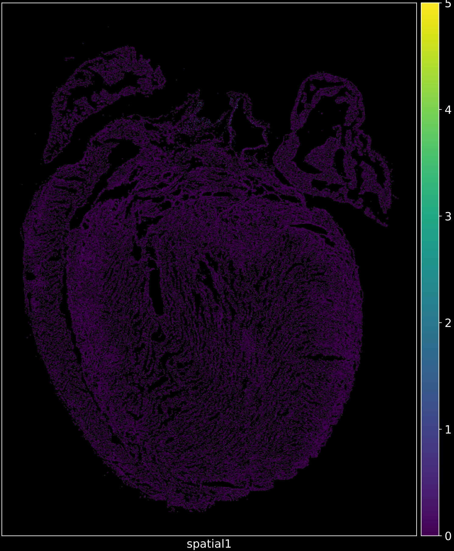
Cnn1 in KO1
