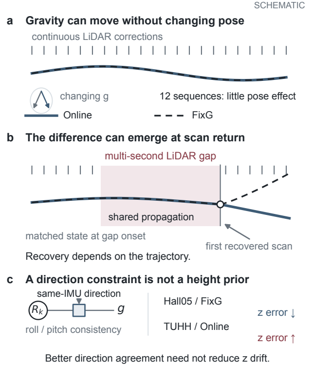
Fig. 1. Study logic (schematic, not measured paths). a , Continuous LiDAR correction can mask gravity-state motion. b , Matched states share propagation; scan return can reveal different recovery. c , A direction factor from the same IMU constrains attitude, not height: the tested dropout cases show opposite vertical-error responses.
