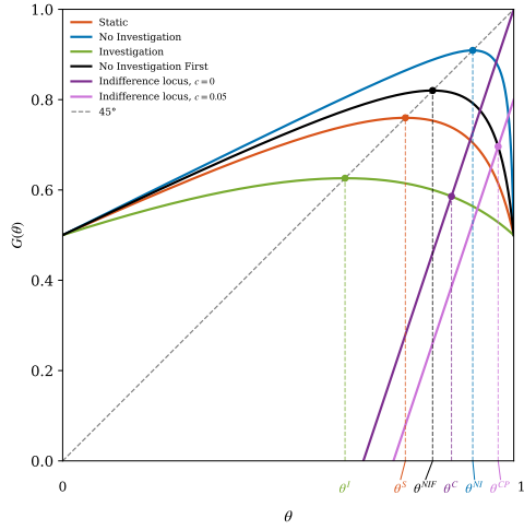
(a) p = 0.1, g = 0.2, c = 0.05 . Five regimes, with \theta^I < \theta^S < \theta^{NIF} < \theta^C < \theta^{NI} < \theta^{CP}
