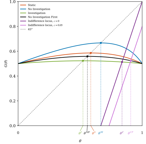
(b) p = 0.5, g = 0.2, c = 0.05 . Five regimes, with \theta^I < \theta^{NIF} < \theta^S < \theta^{NI} < \theta^C < \theta^{CP}
