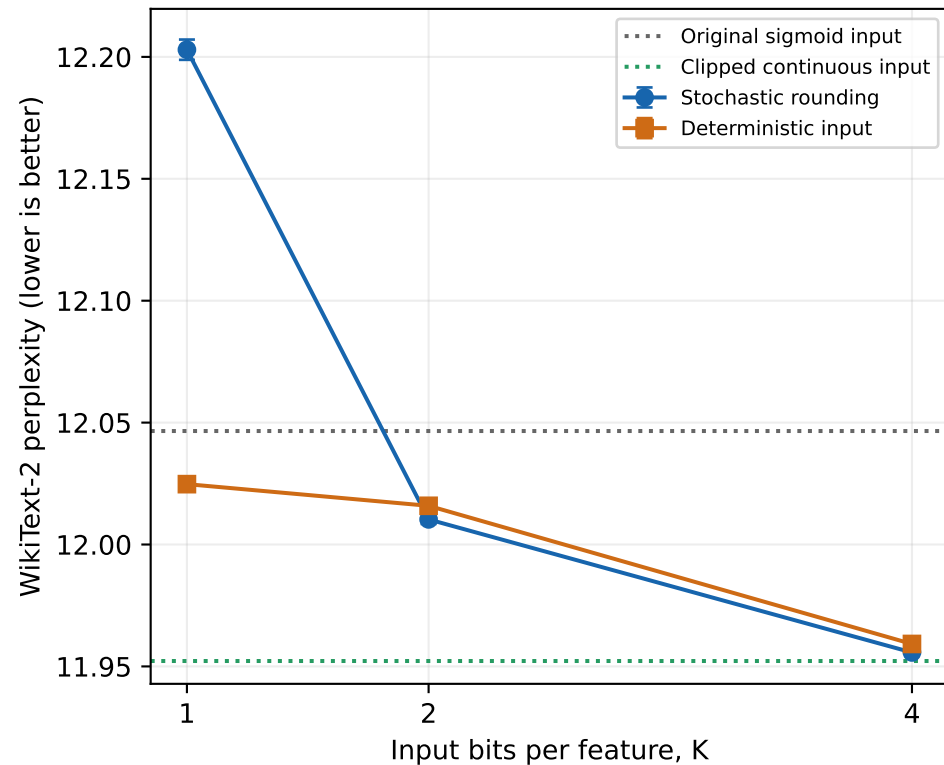
Full-model quality, N=4
