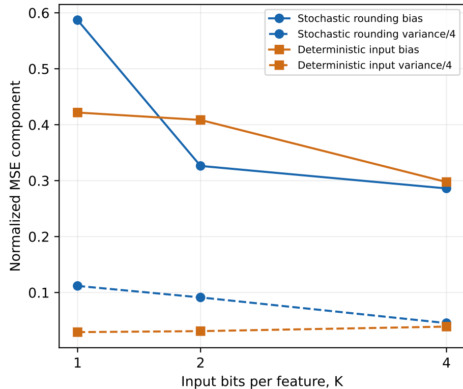
Trained FFN output error
