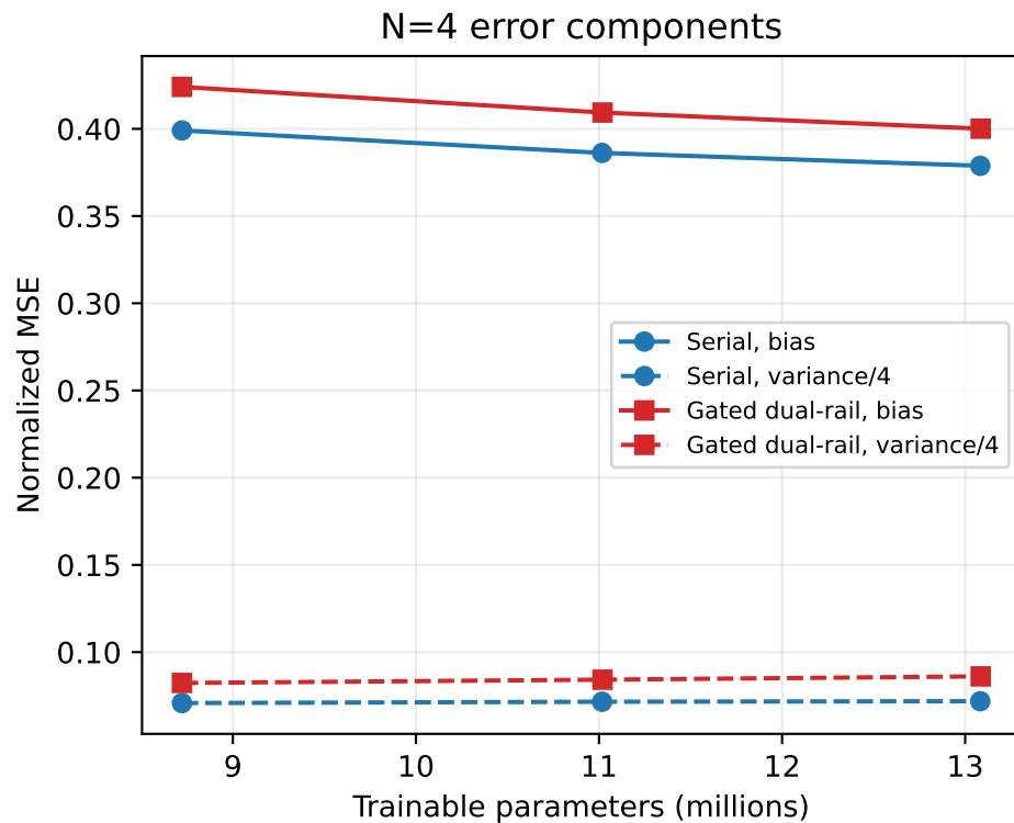
0/1 p-bit FFN width sweep, Qwen2.5-0.5B layer 12
