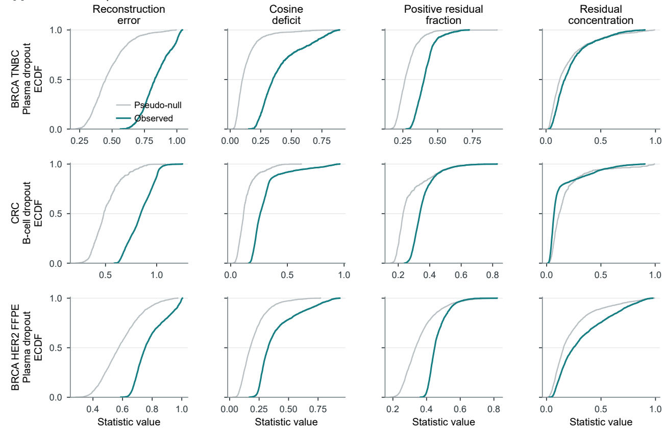
A Observed vs pseudo-null calibration
