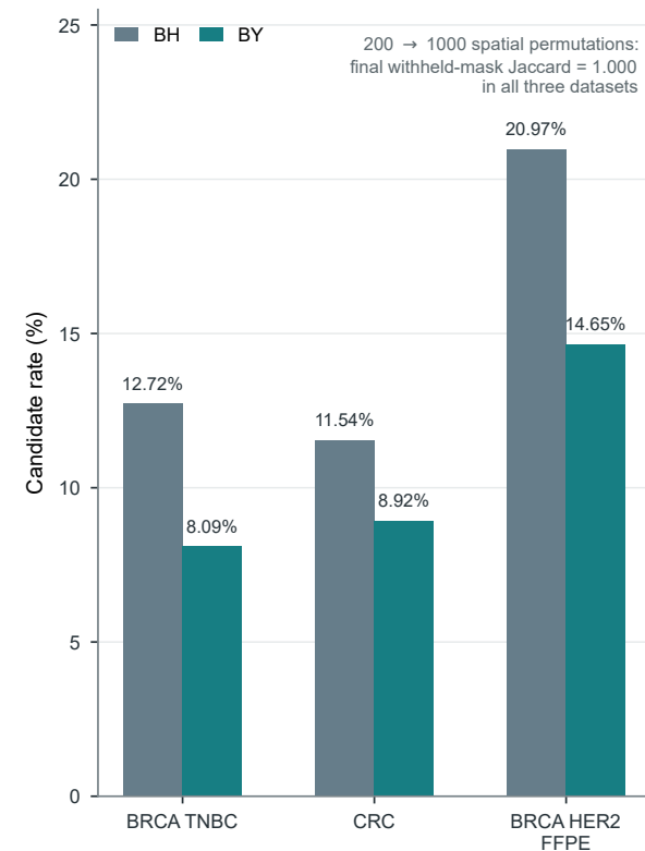
C Statistical robustness
