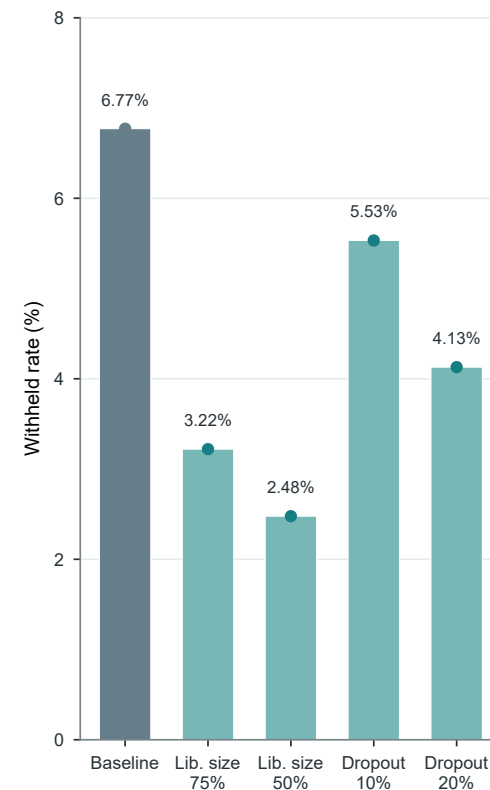
B Technical perturbation control
