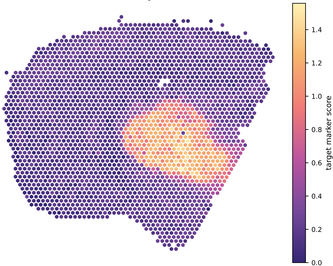
Thalamic excitatory marker score
