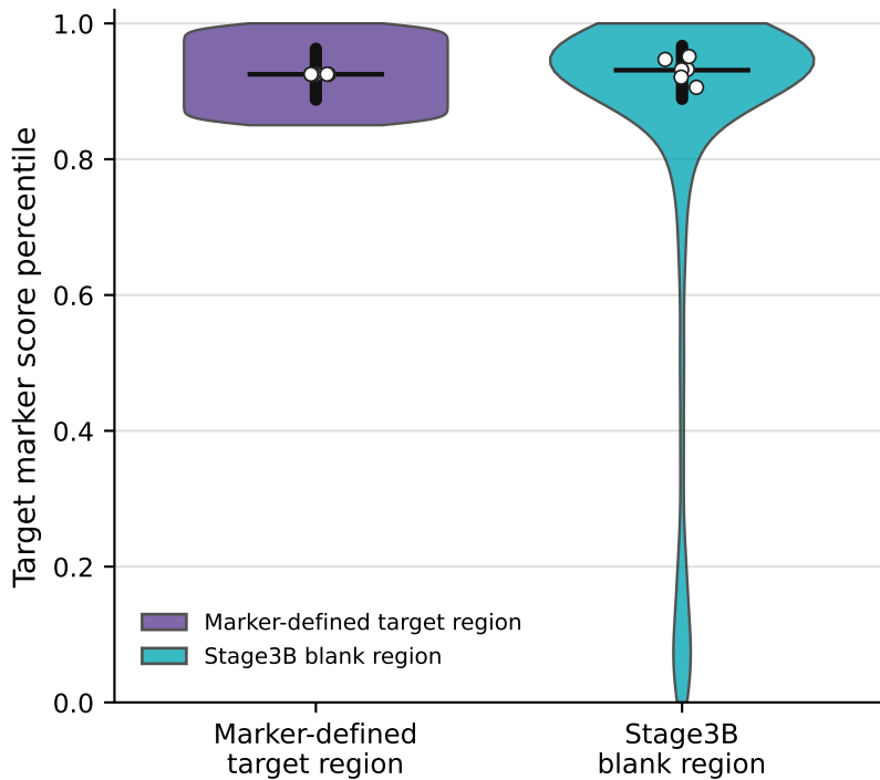
Panel A Stage3B blank regions preserve target-marker enrichment
