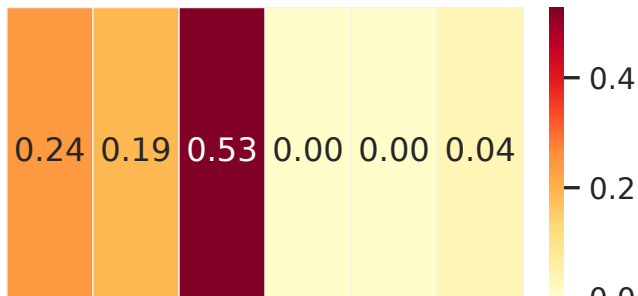
B. CytoSPACE forced assignment of ST-only region
