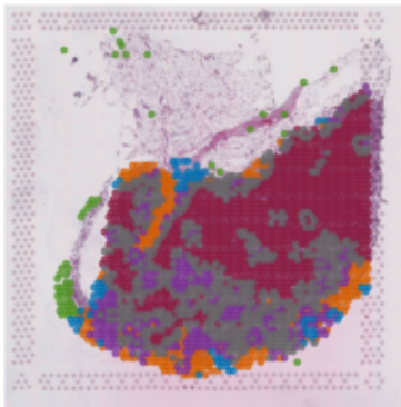
Unsupervised local niches
