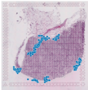
SVTuner withheld-positive spots
