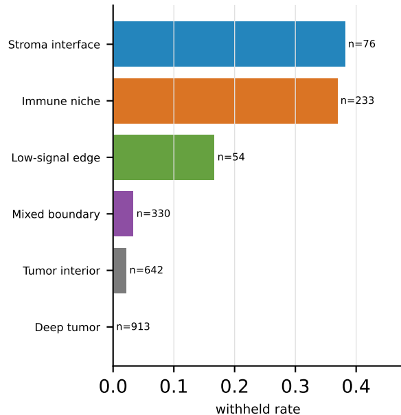
Withheld enrichment by niche
