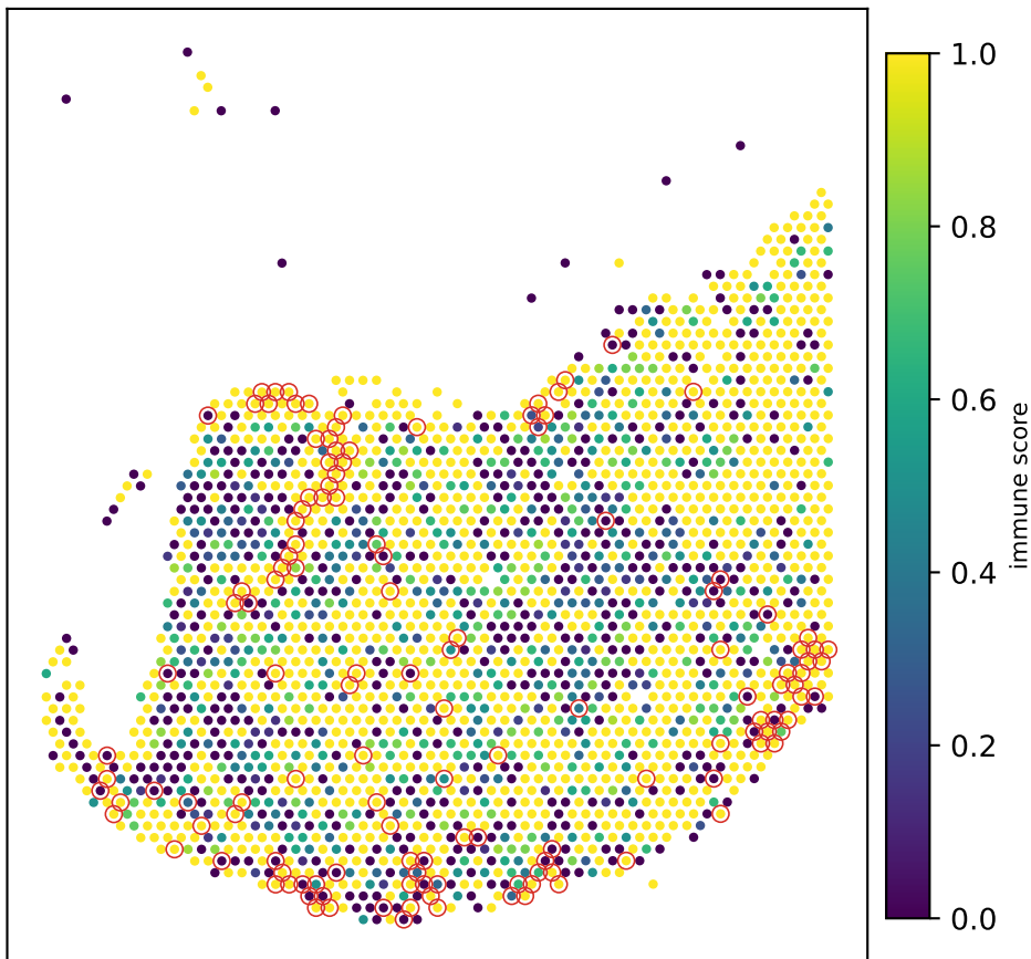
full reference
