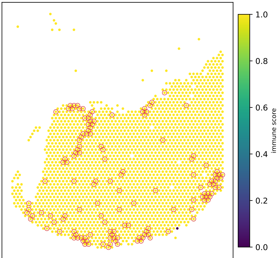
nonimmune all dropout control
