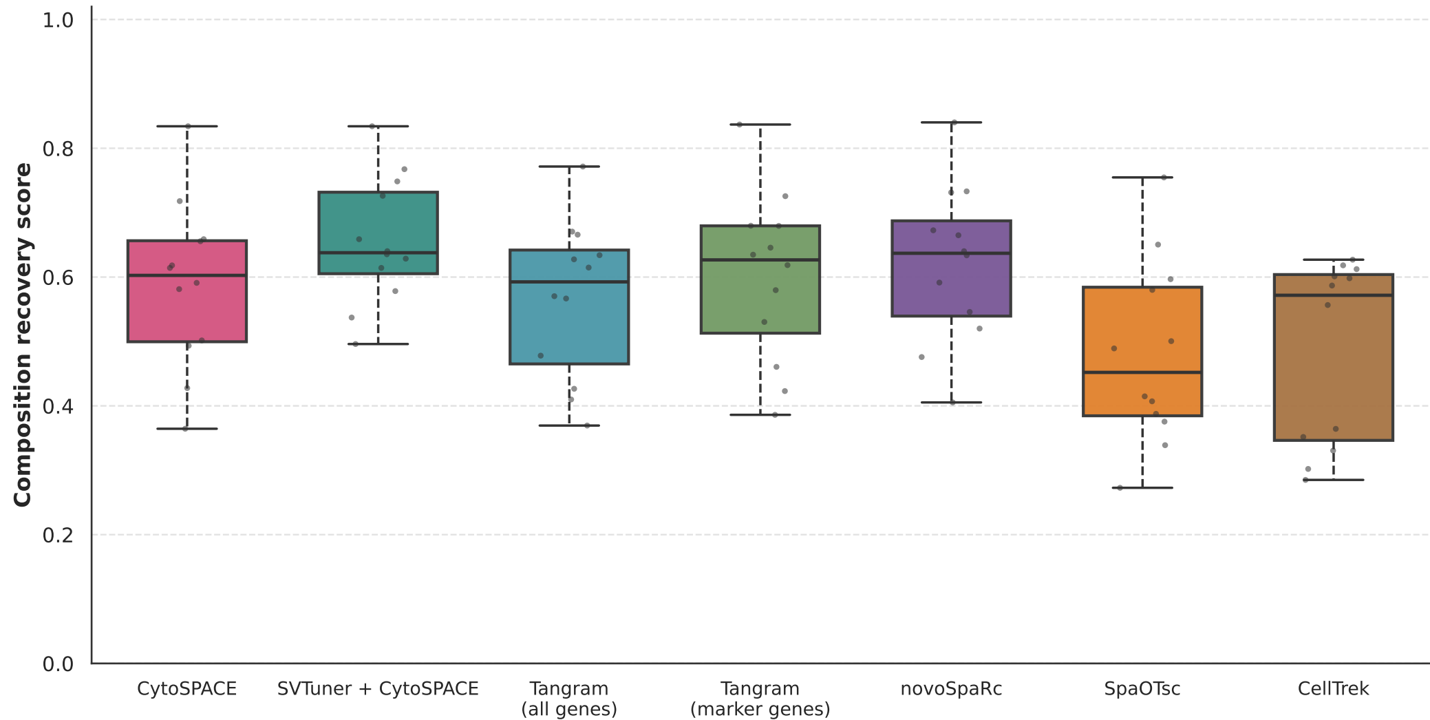
Spatial cell-type composition recovery, 10% sc noise
