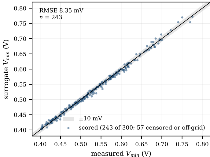
read (SNM, 125 °C)
