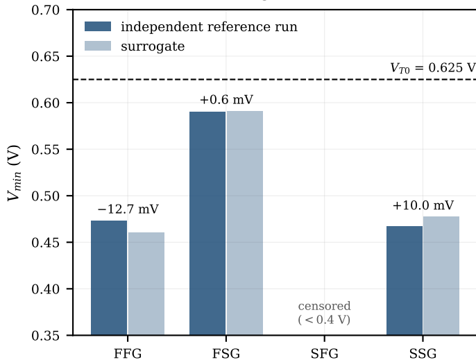
read @ 125 °C
