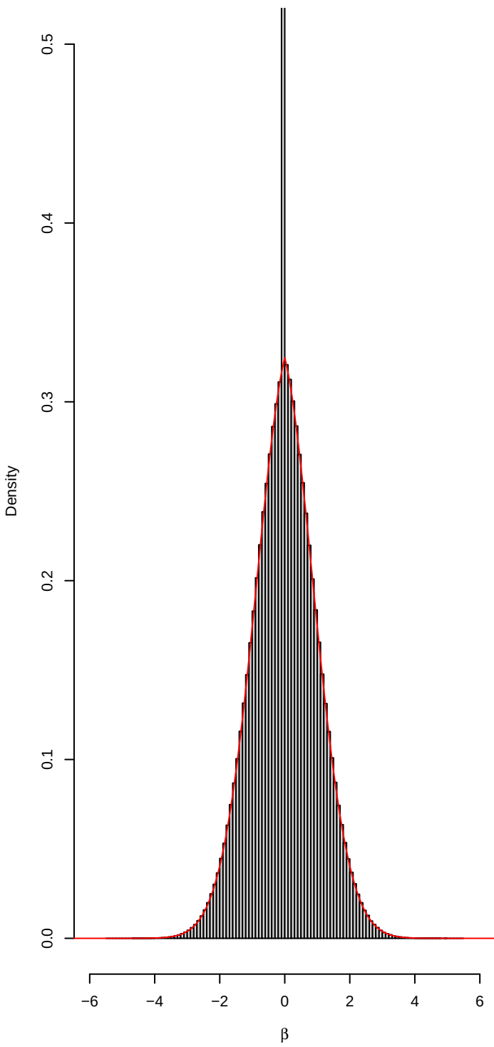
P(\beta = 0) = 0.25
