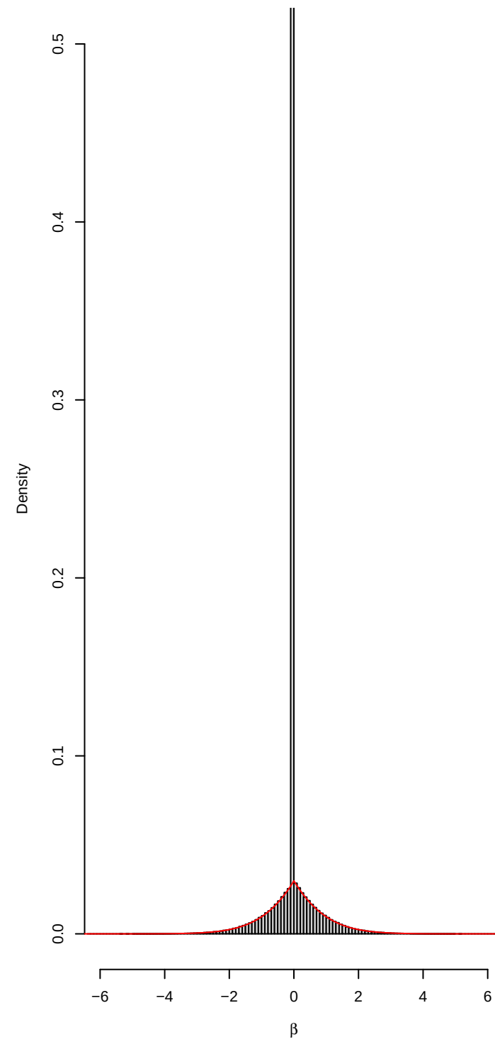
P(\beta = 0) = 0.95
