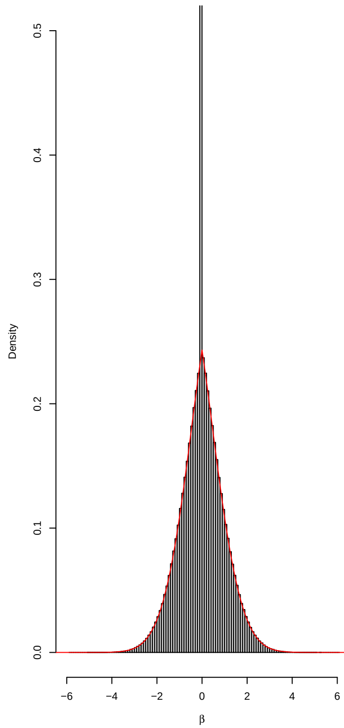
P(\beta = 0) = 0.5
