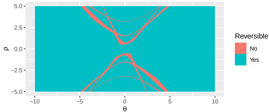
N(0, 1) – RKNF criterion – L = 1 , h = \pi / 2 , \delta = 1
