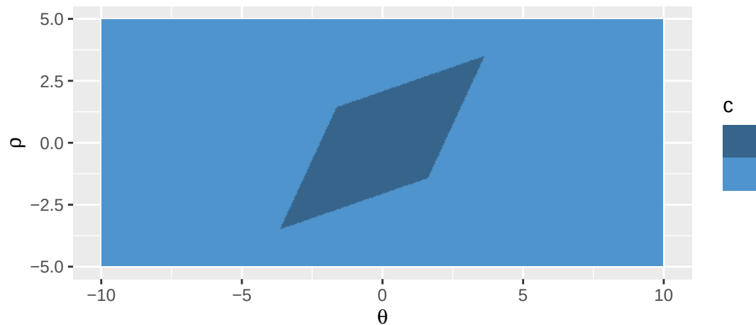
N(0, 1) – MRF criterion – L = 1 , h = \pi / 2 , \delta = 1
