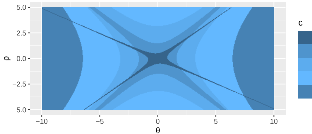
N(0, 1) – RKNF criterion – L = 1 , h = \pi / 2 , \delta = 1
