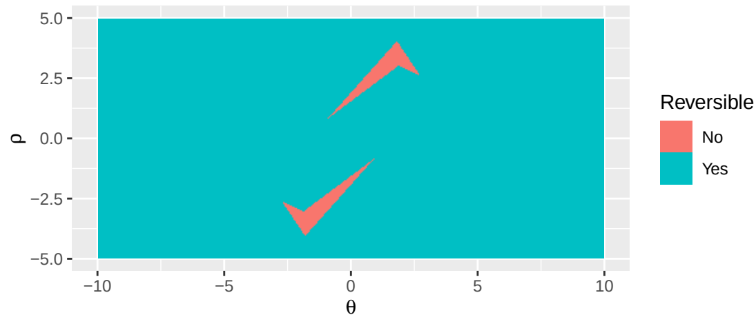
N(0, 1) – MRF criterion – L = 1 , h = \pi / 2 , \delta = 1
