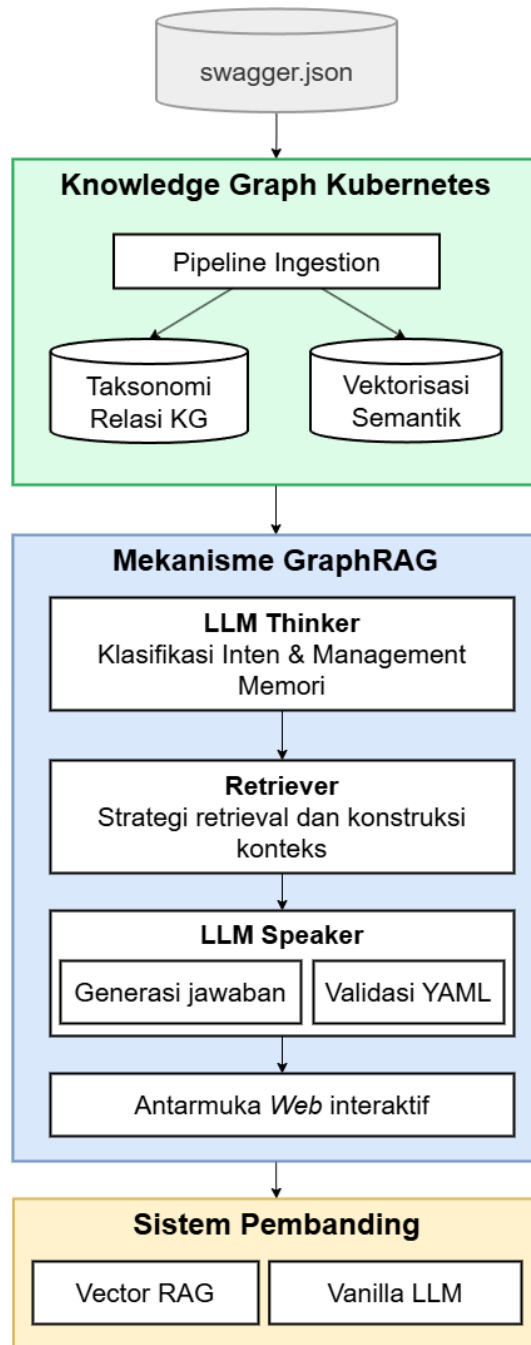
Gambar IV.2 Architecture Diagram Sistem GraphRAG Kubernetes
