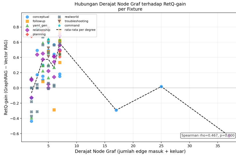
Gambar VI.3 Scatter plot derajat node primer vs. RetQ-gain . Korelasi Spearman \rho = +0,467 ( p < 0,001 , n = 96 ).
