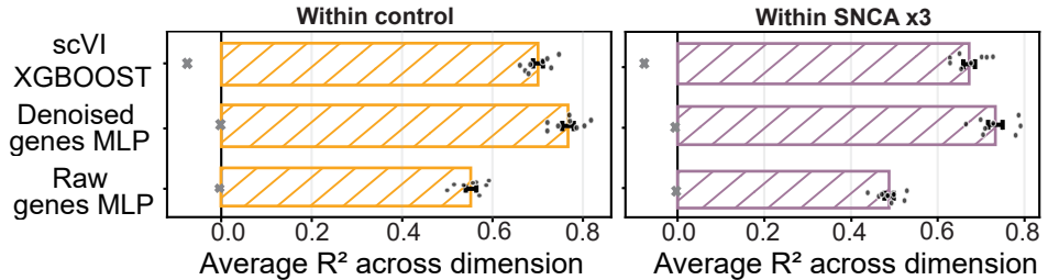
(b) Dimension Averaged Predictability Under GW-map
