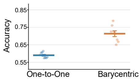
(a) Gromov-Wasserstein Coupling Accuracy
