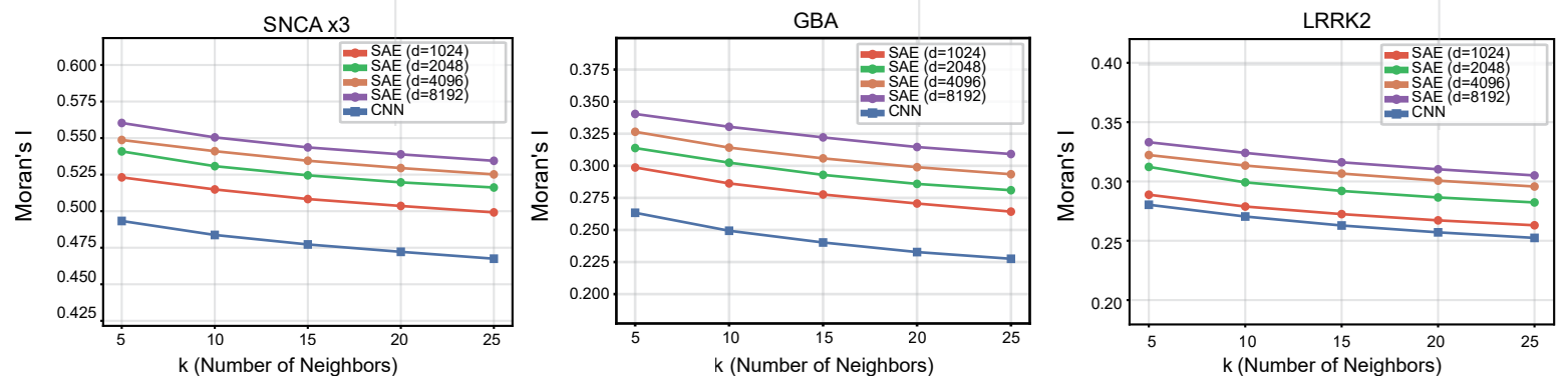
(b) Moran's I of cell death per mutation
