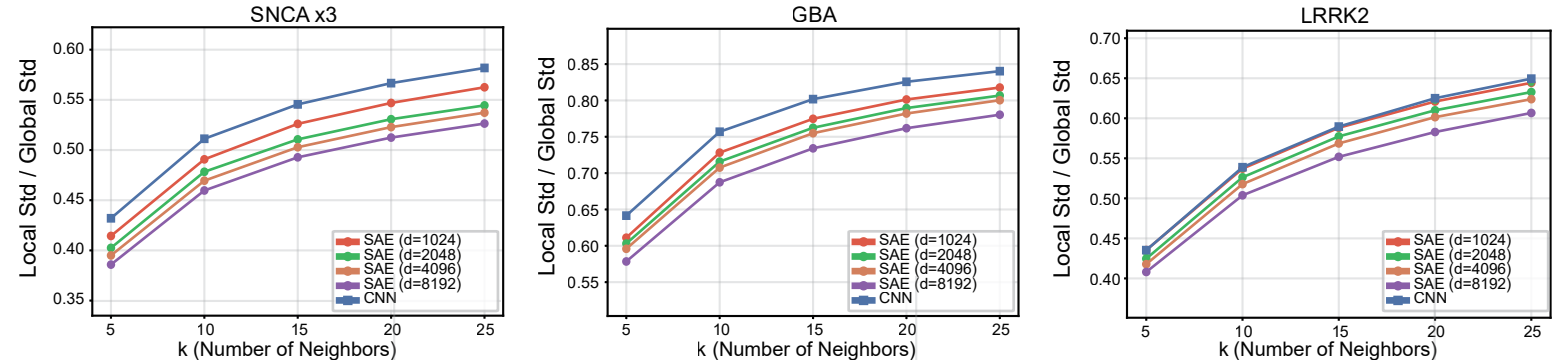
(a) Ratio of the mean local SD to the global SD of cell death rates per mutation
