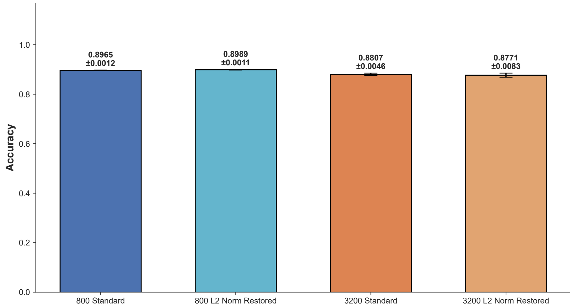
SAE Probe Accuracy Comparison (stage5_out)
