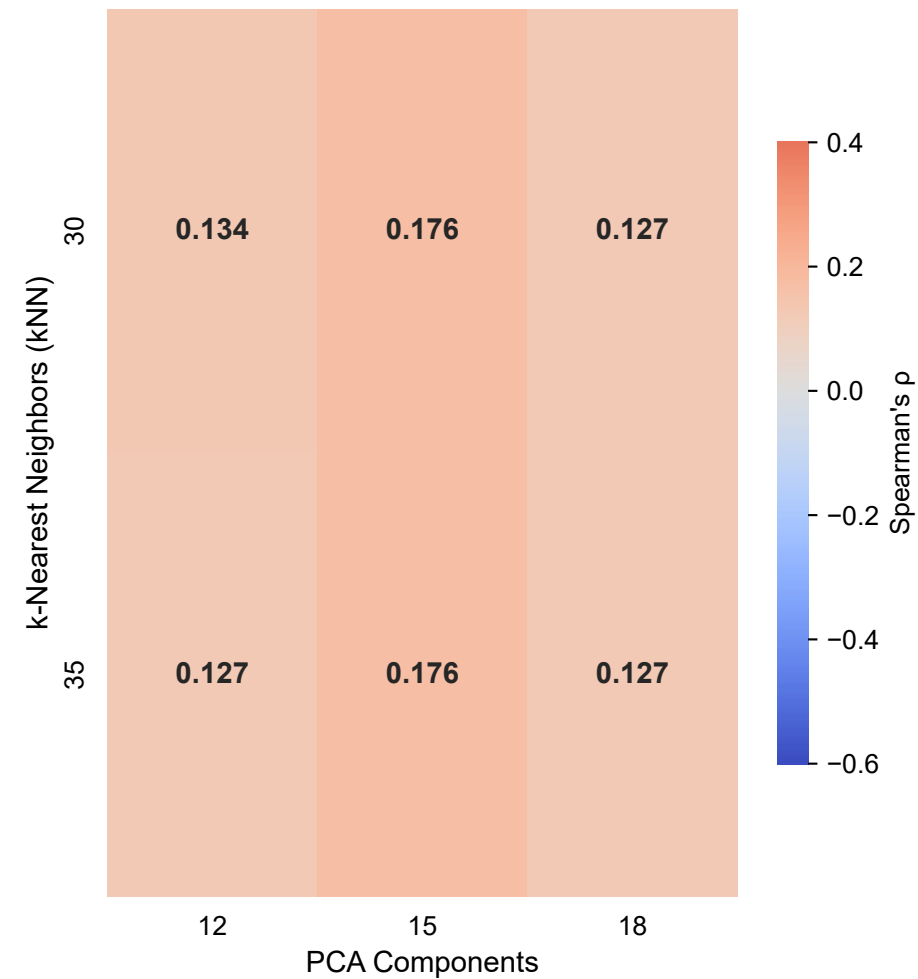
SAE Mutation: LRRK2
