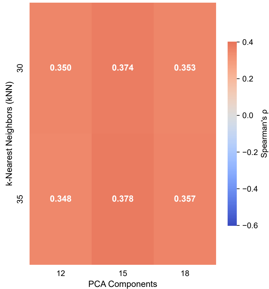
SAE Mutation: SNCA
