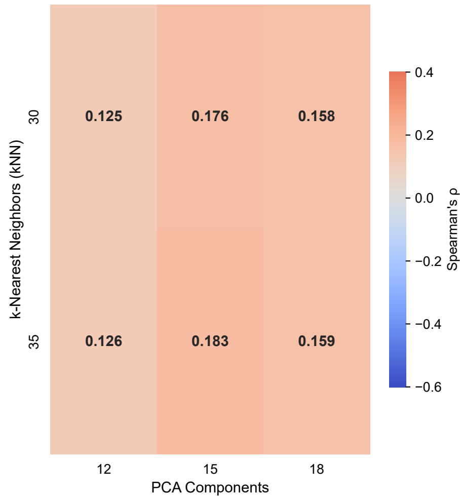
SAE Mutation: GBA
