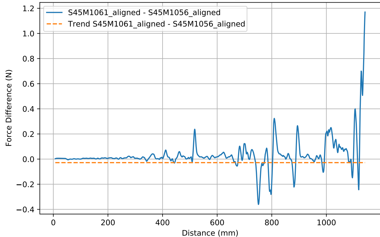
Interpolated Drift Difference: S45M1061_aligned - S45M1056_aligned
