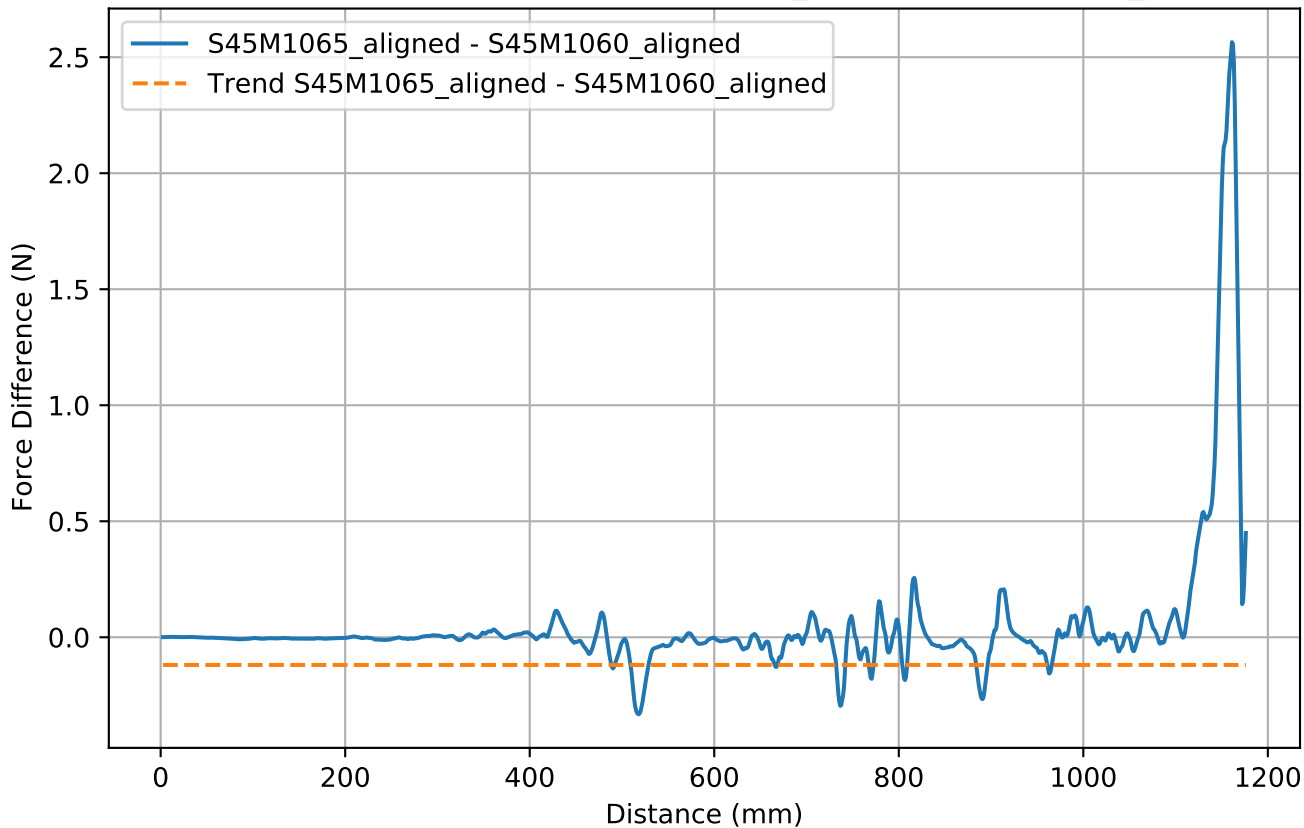
Interpolated Drift Difference: S45M1065_aligned - S45M1060_aligned
