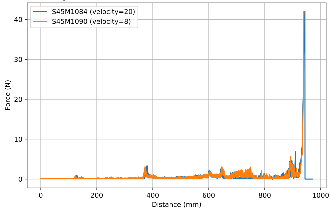
Signal shifted with cross-Correlation S45M1090 & S45M1084
