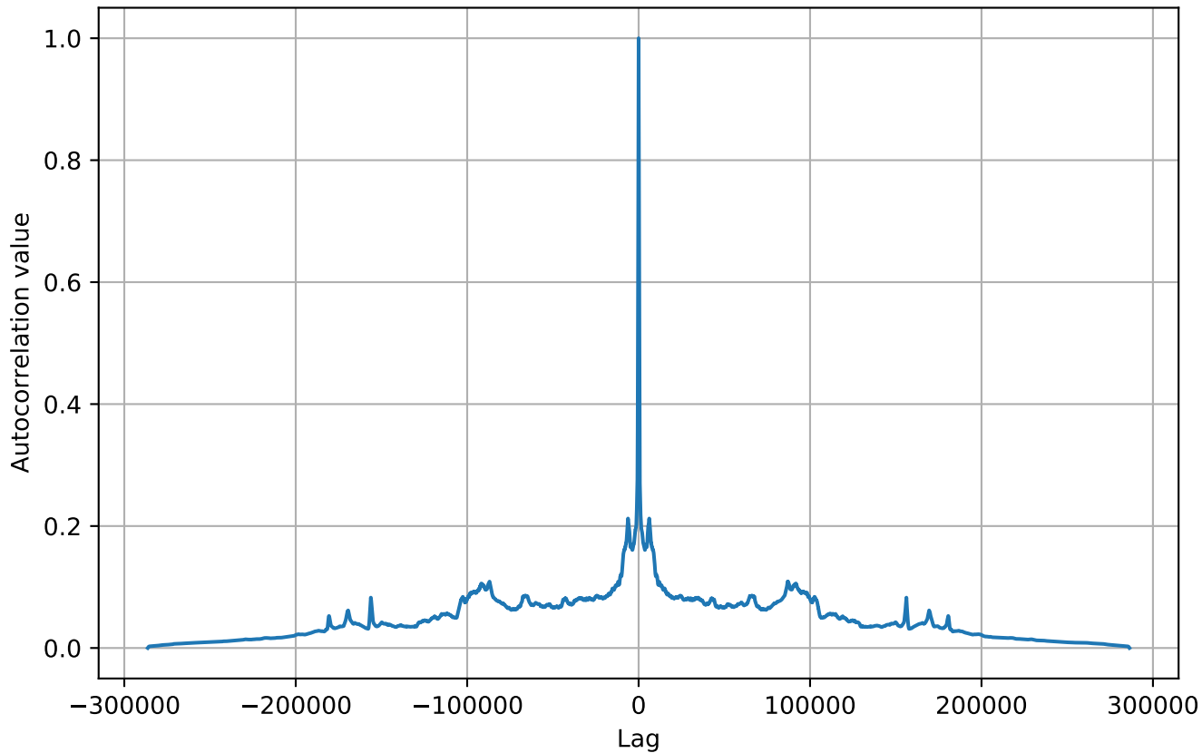
Autocorrelation: S45M1064
