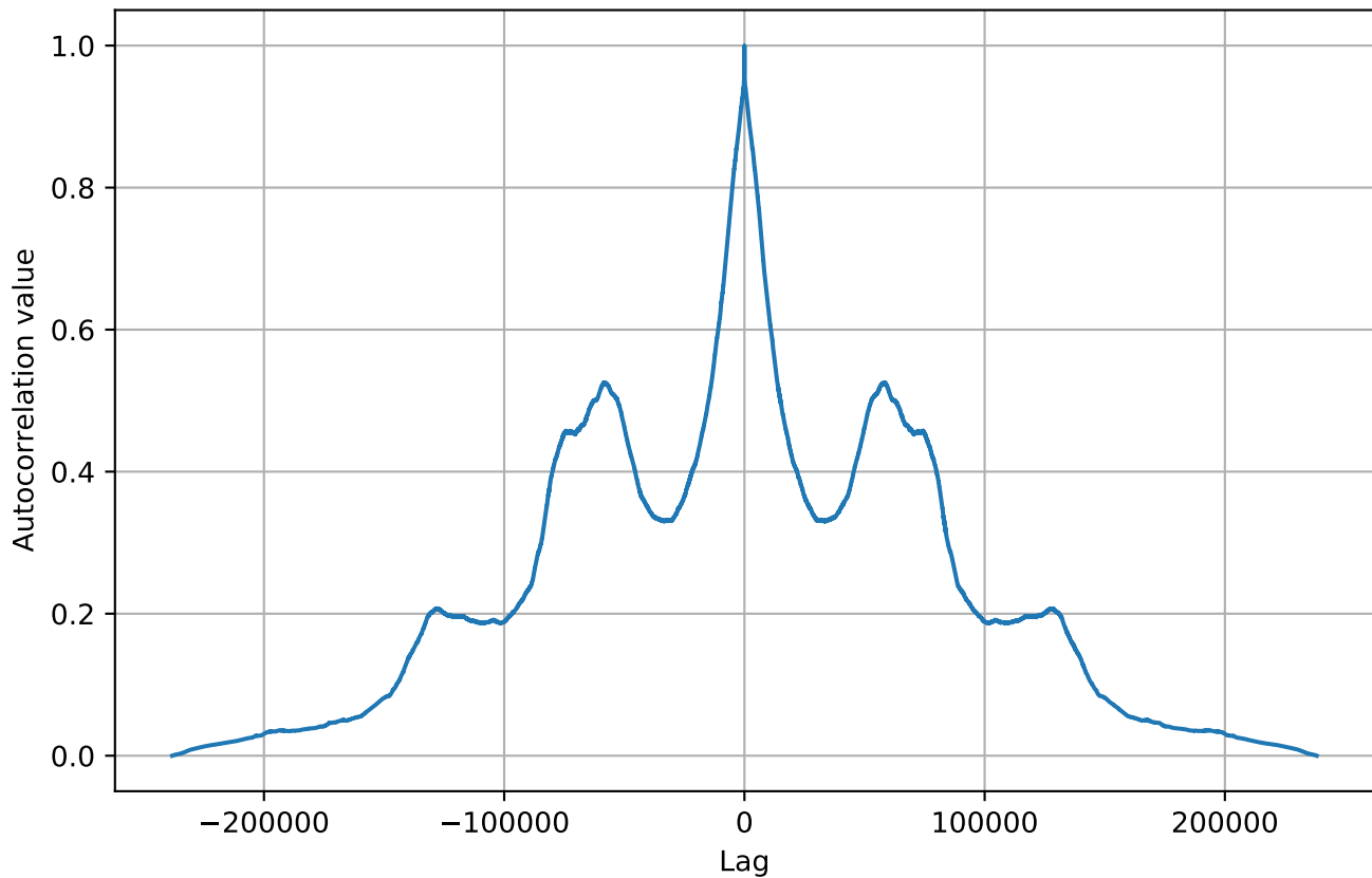
Autocorrelation: S45M1087
