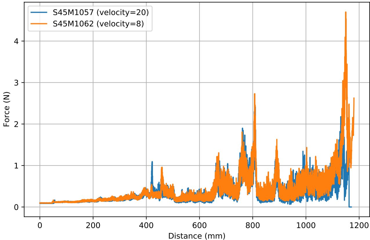
Signal shifted with cross-Correlation S45M1062 & S45M1057
