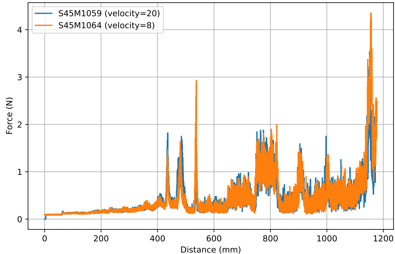
Signal shifted with cross-Correlation S45M1064 & S45M1059
