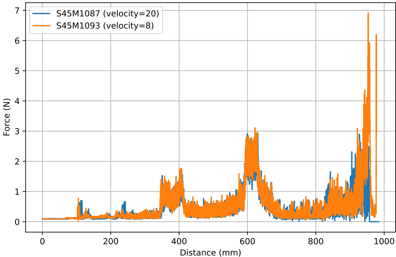
Signal shifted with cross-Correlation S45M1093 & S45M1087
