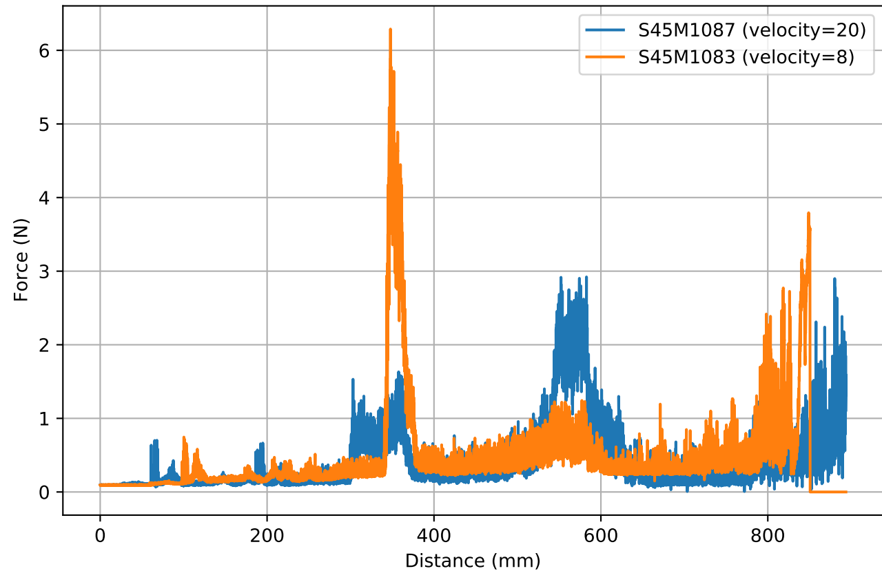
Aligned: S45M1087 to S45M1083 (Day 2)
