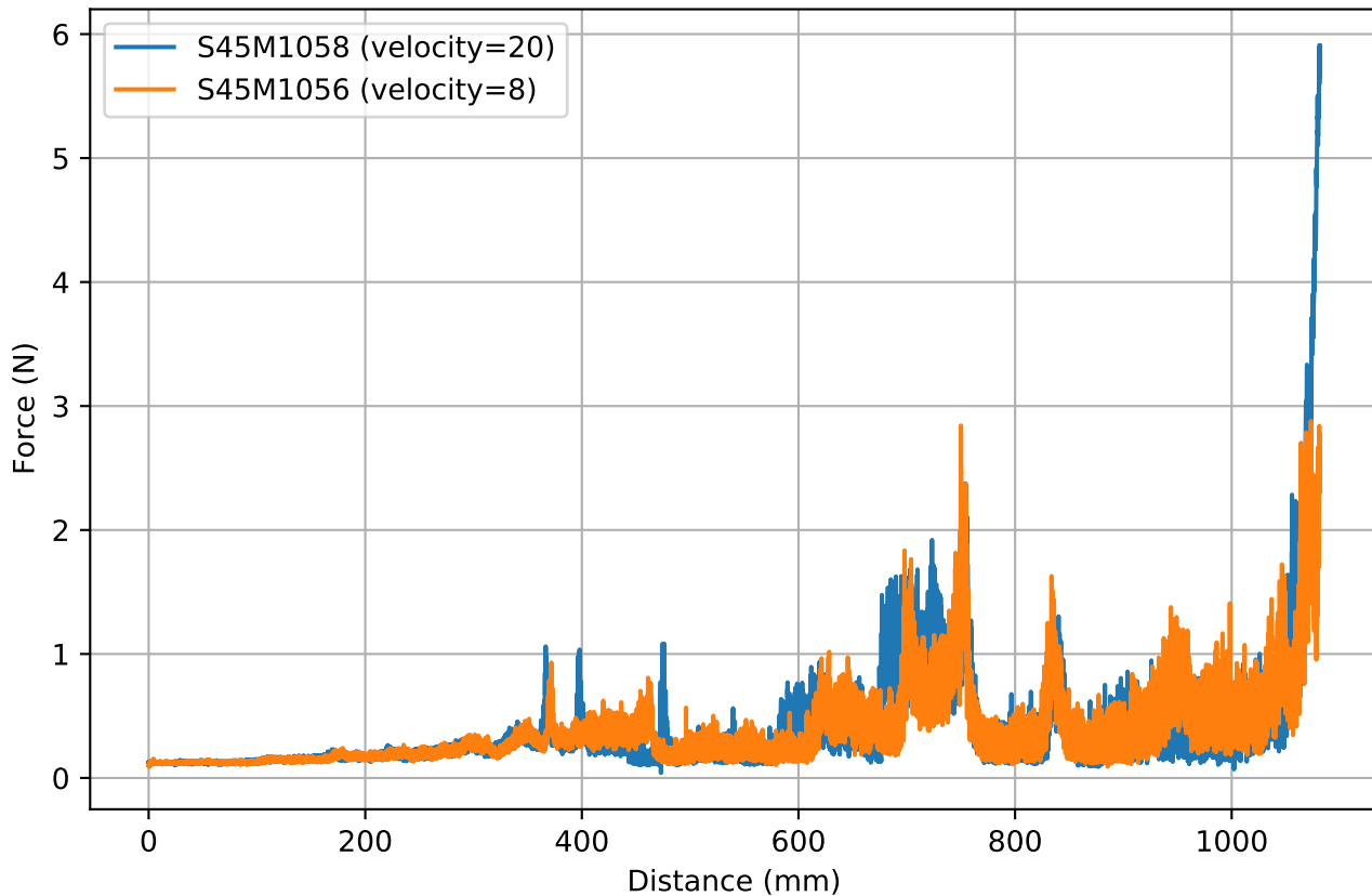
Signal shifted with cross-Correlation S45M1056 & S45M1058
