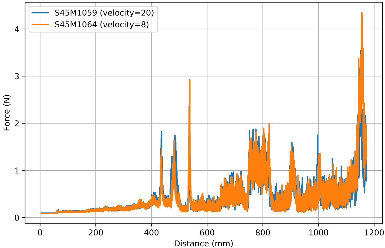
Signal shifted with cross-Correlation S45M1064 & S45M1059
