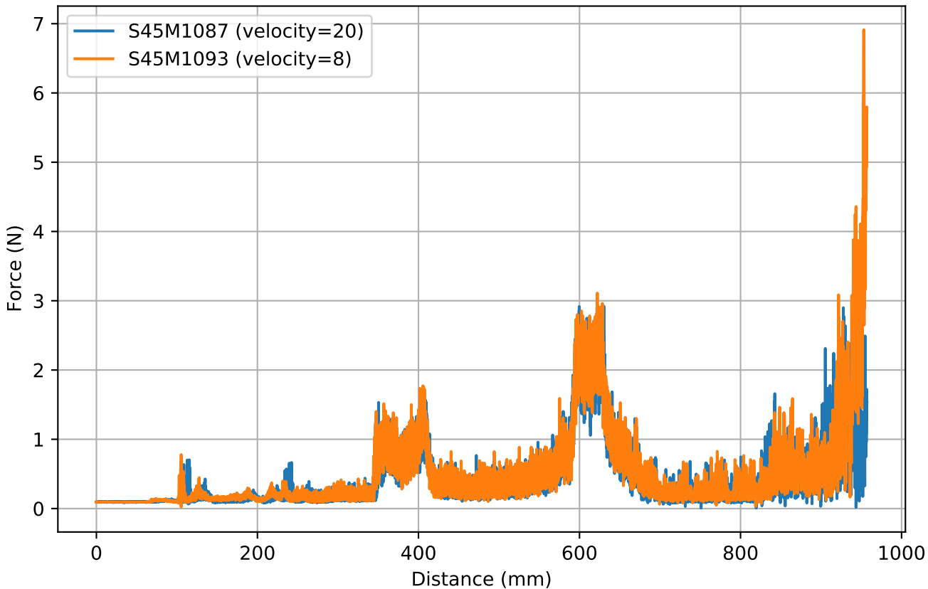
Signal shifted with cross-Correlation S45M1093 & S45M1087
