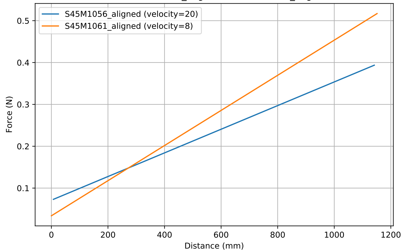
Trend S45M1061_aligned vs S45M1056_aligned
