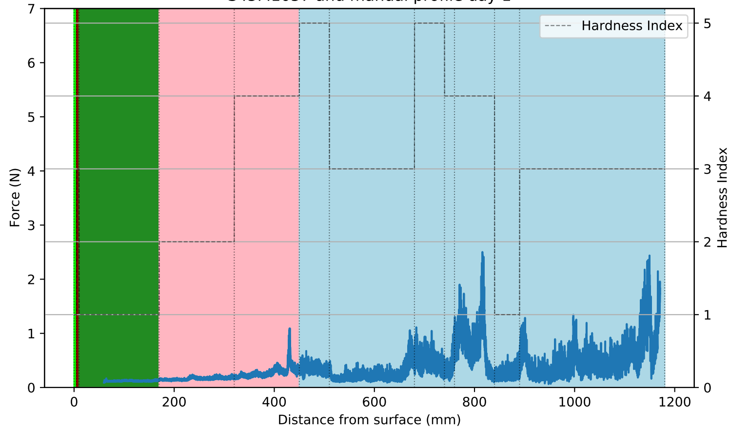
S45M1057 and manual profile day 1
