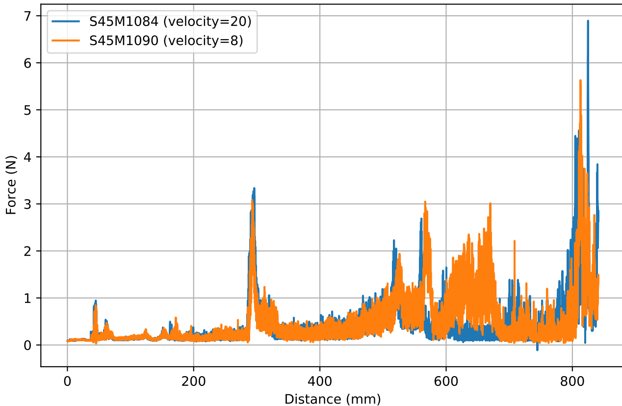
Signal shifted with cross-Correlation S45M1090 & S45M1084
