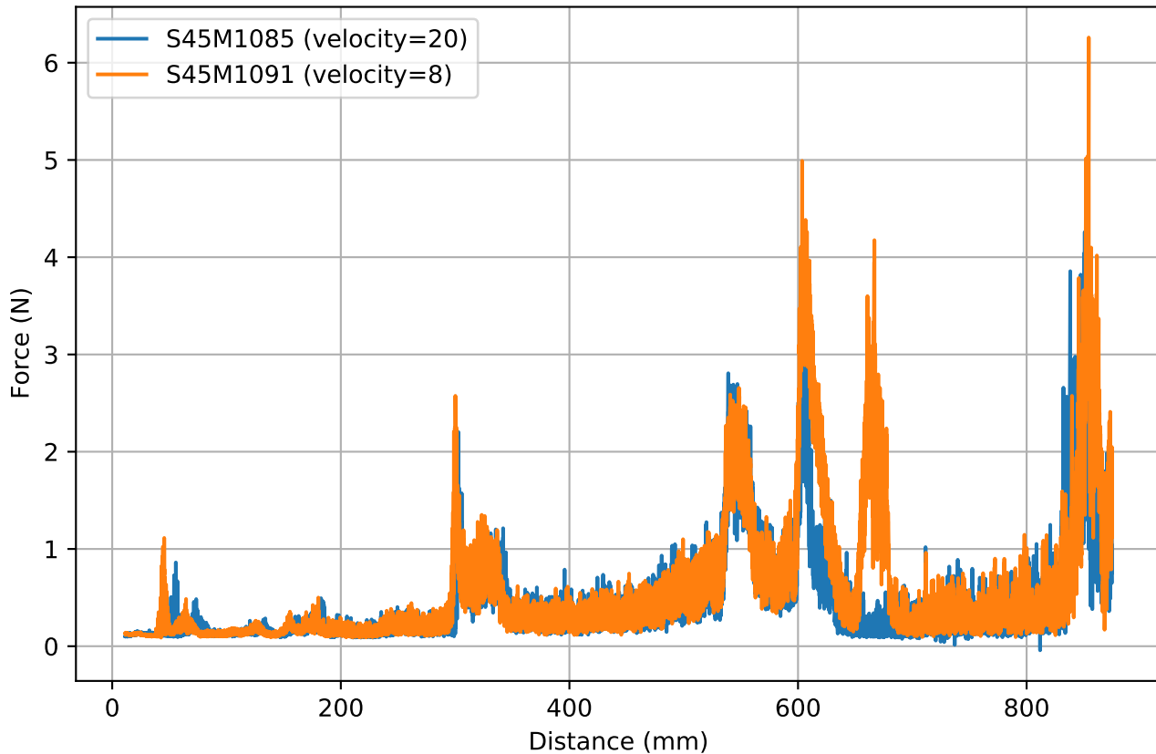
Signal shifted with cross-Correlation S45M1091 & S45M1085
