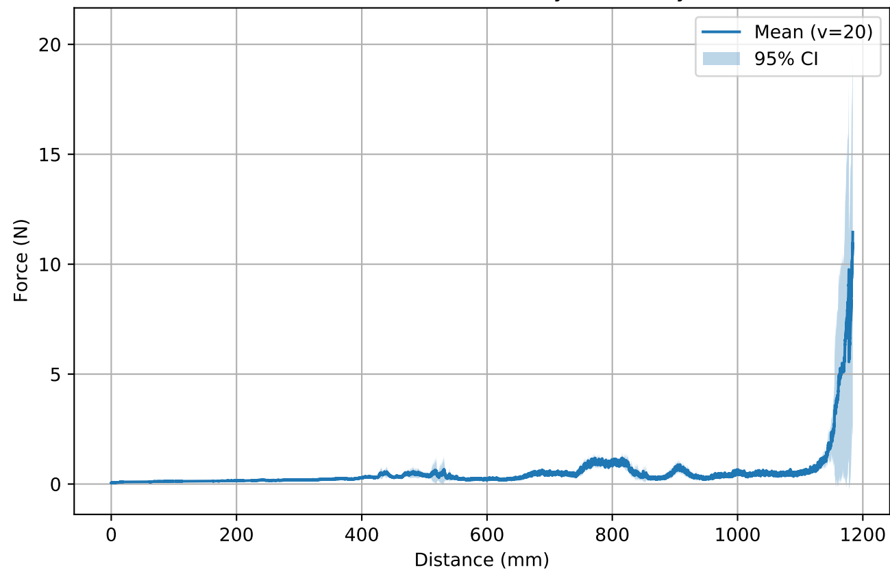
Mean Profile with 95% CI Day 1, Velocity 20
